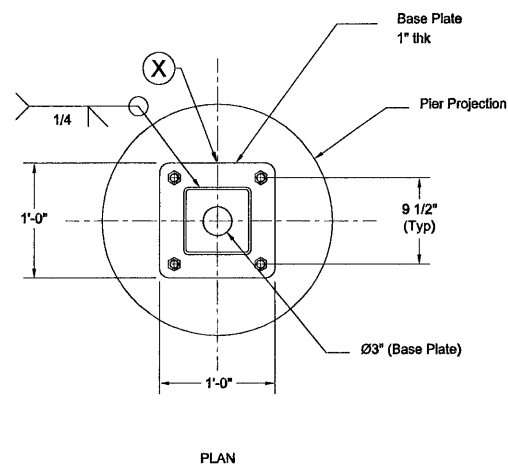
PIER DETAIL - P3
