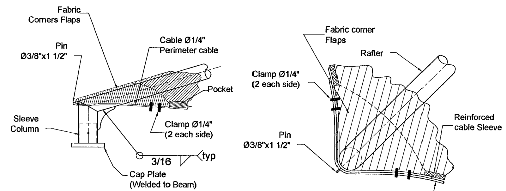
TYPICAL FABRIC ATTACHMENT DETAIL H
