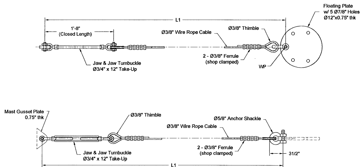
TYPICAL CABLE ASSEMBLY DETAIL (TCA1) (MAST - FLOATING PLATE)
