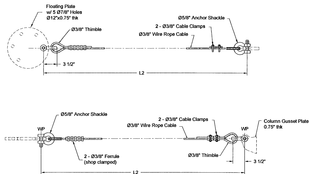
TYPICAL CABLE ASSEMBLY DETAIL (TCA2) (FLOATING PLATE - COLUMN)
