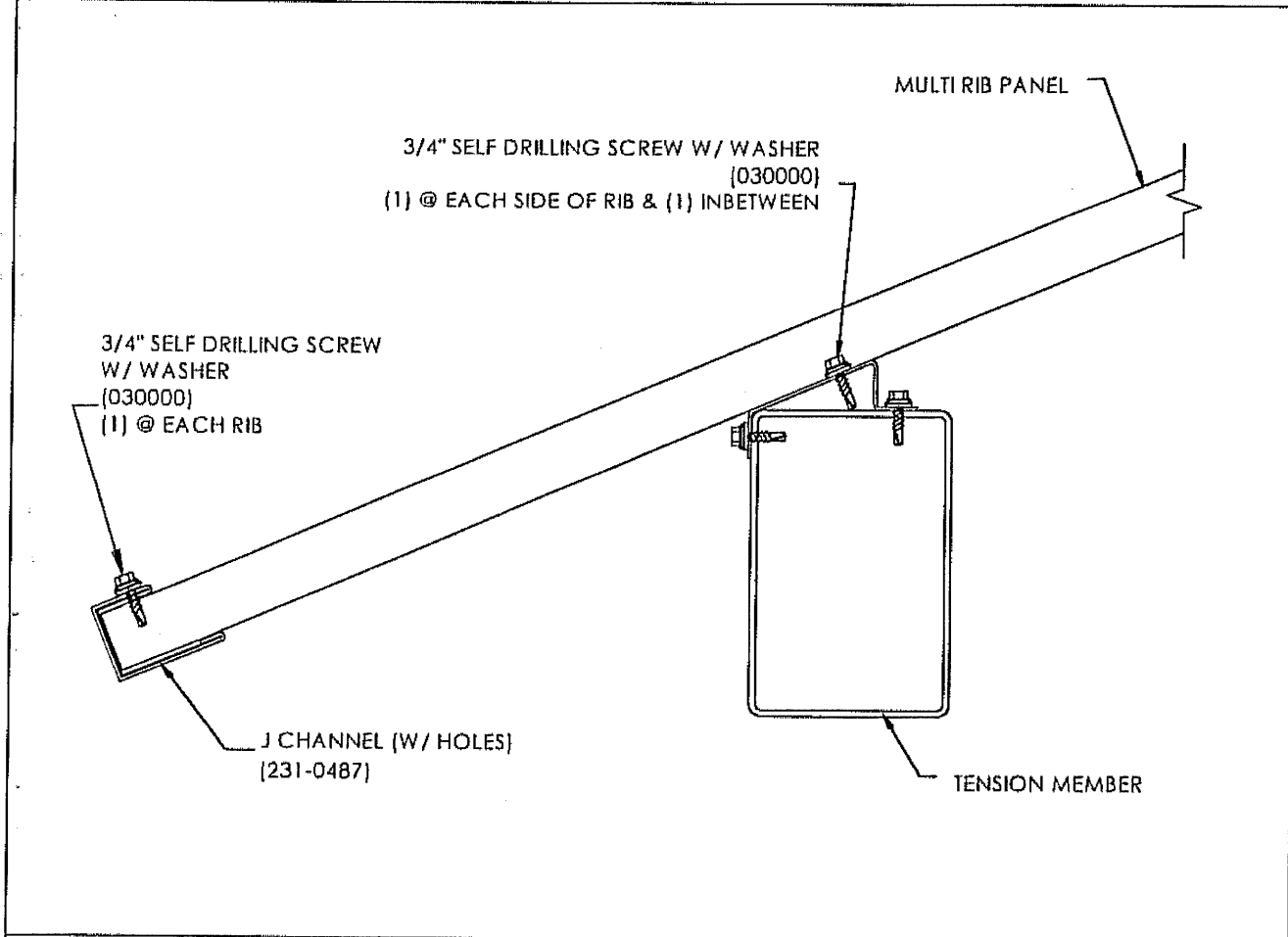
SECTION @ EAVE
