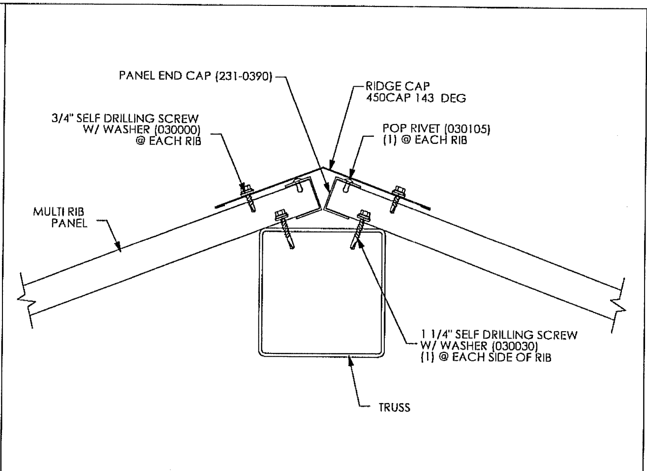
SECTION @ TRUSS
