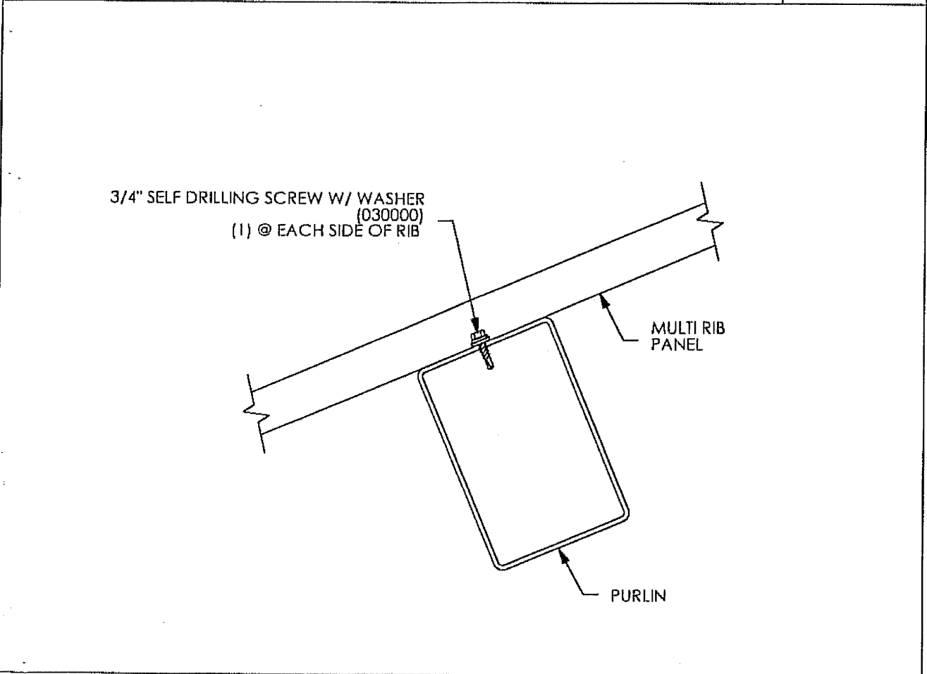
SECTION @ PURLIN
