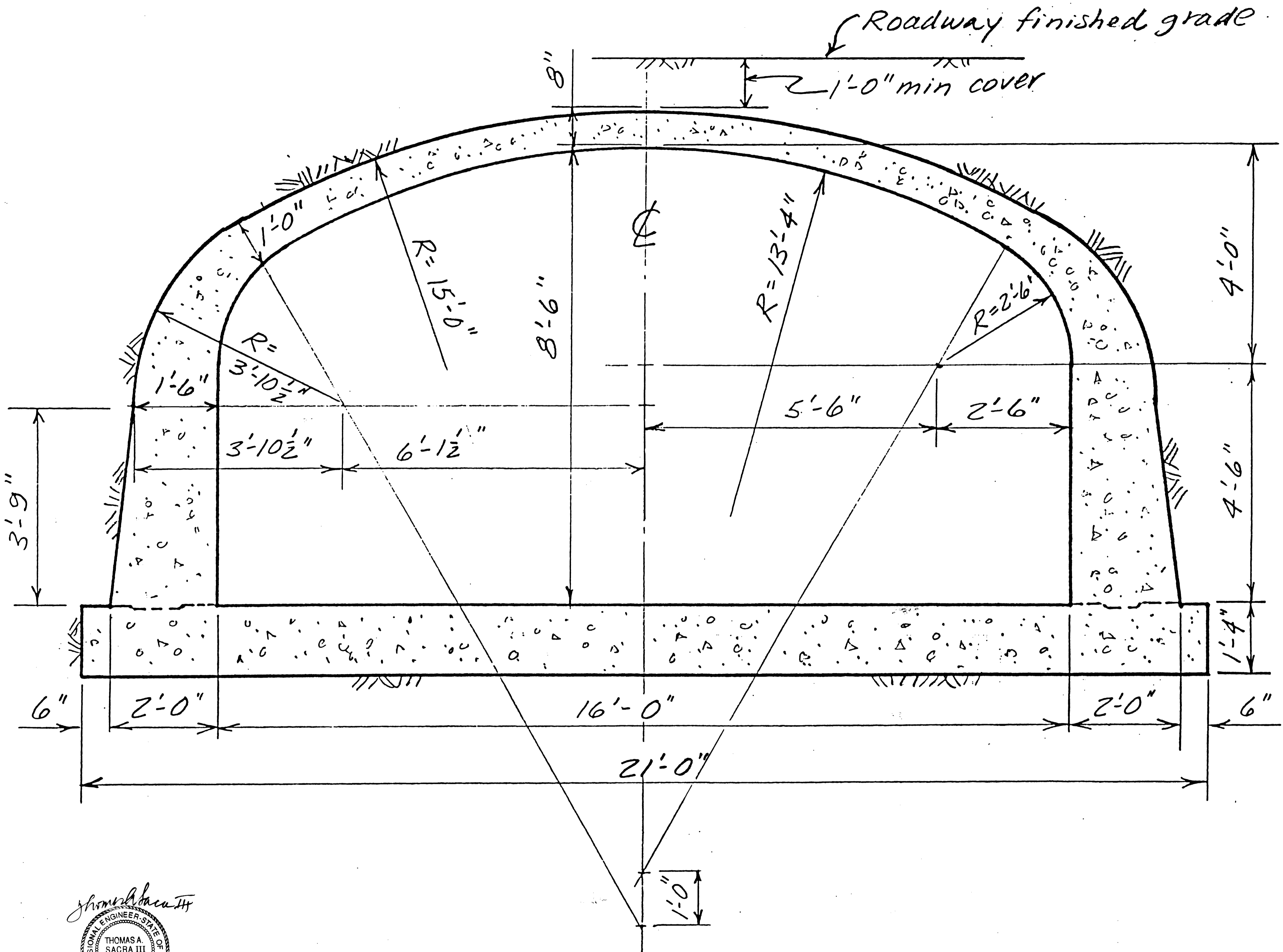
CROSS-SECTION GEOMETRY (B)
