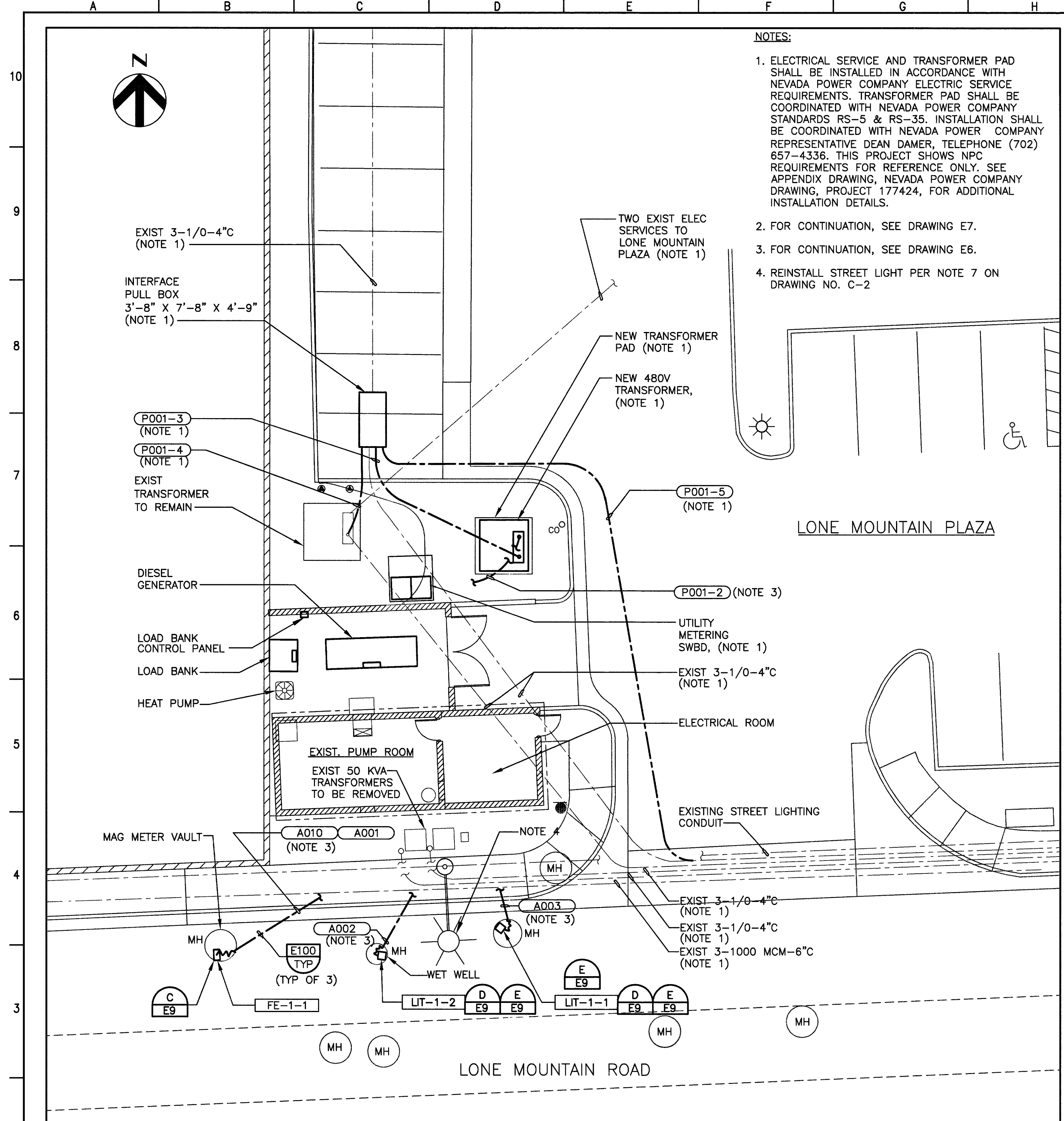
POWER SITE PLAN
