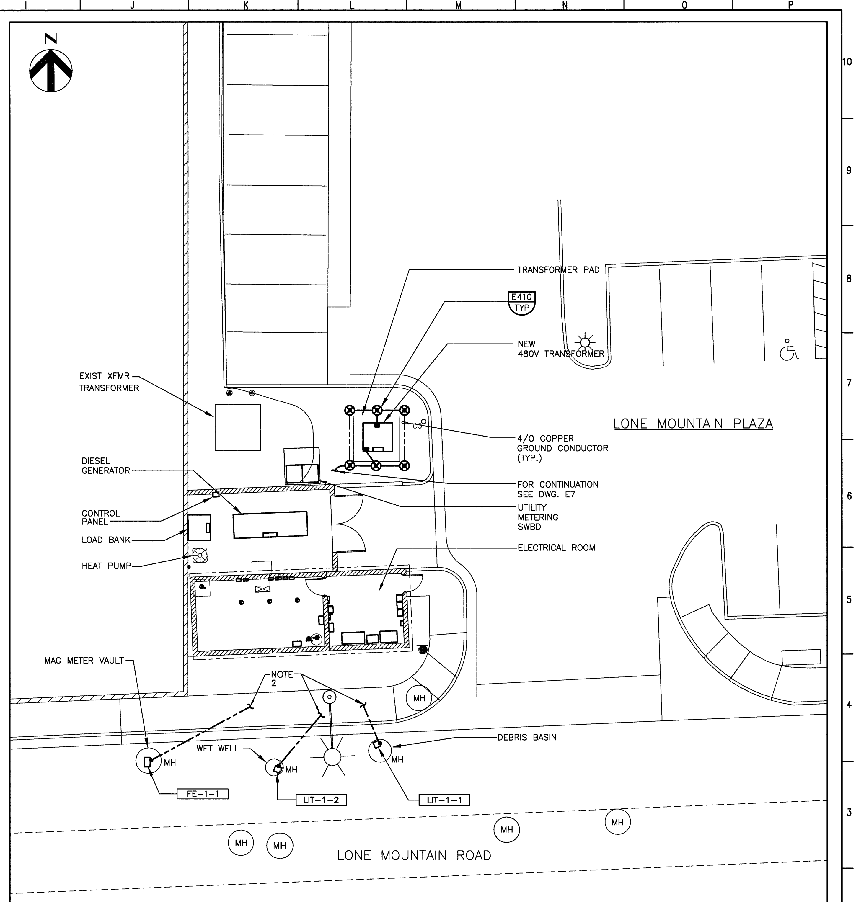
GROUNDING SITE PLAN
