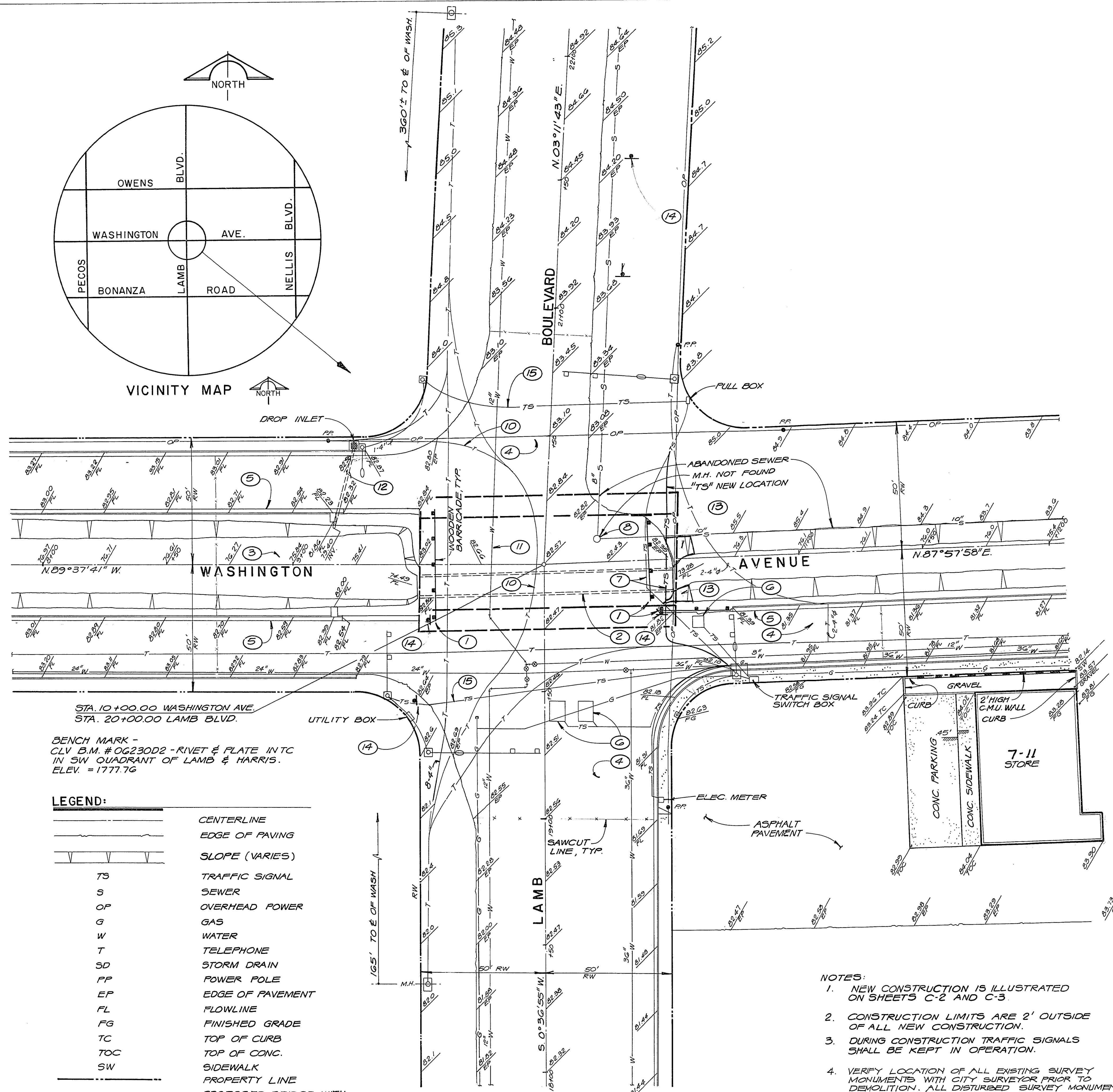
SITE/DEMOLITION PLAN 1"=20'
