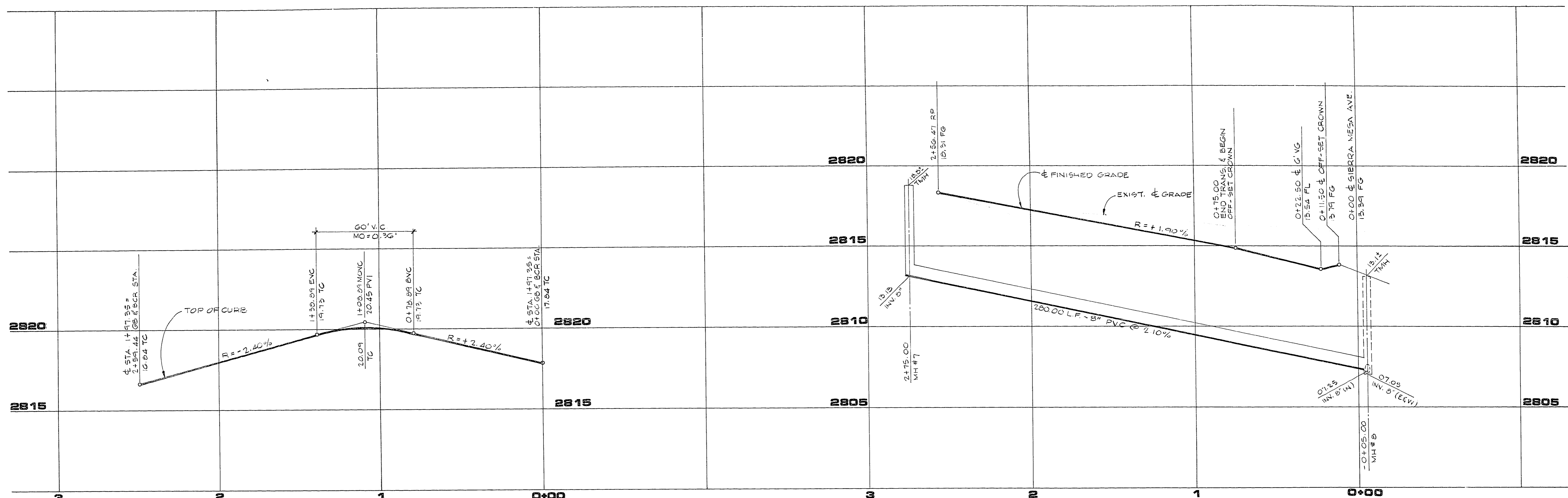
CUL-DE-SAC PROFILE (PEBBLESTONE CIRCLE)
