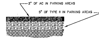
ON-SITE PARKING PAVEMENT SECTION NO SCALE
