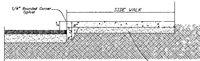
Thickened Edge Walk (ON-SITE ONLY) NO SCALE
