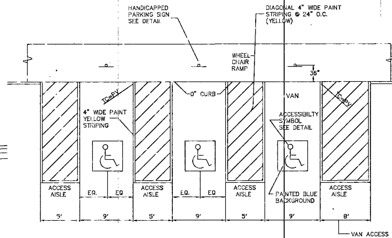
ACCESSIBLE PARKING DETAIL NOT TO SCALE
