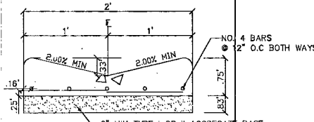
ON-SITE 2' VALLEY GUTTER DETAIL NO SCALE
