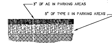
ON-SITE CORRIDOR PAVEMENT SECTION NO SCALE
