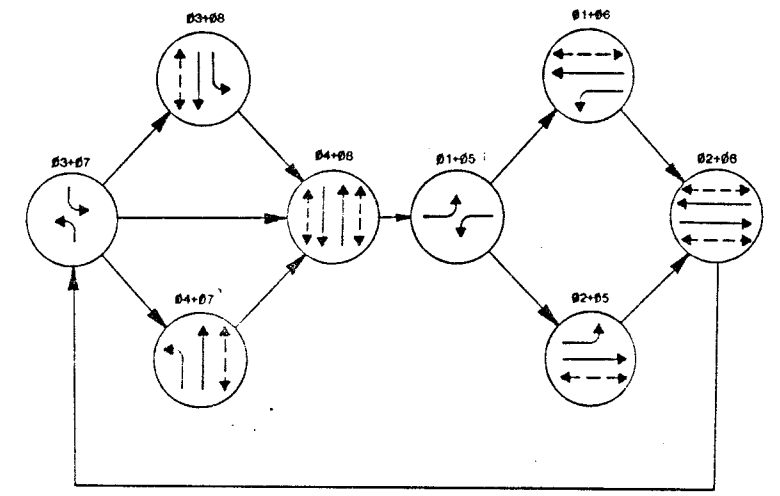
EXISTING PHASING
