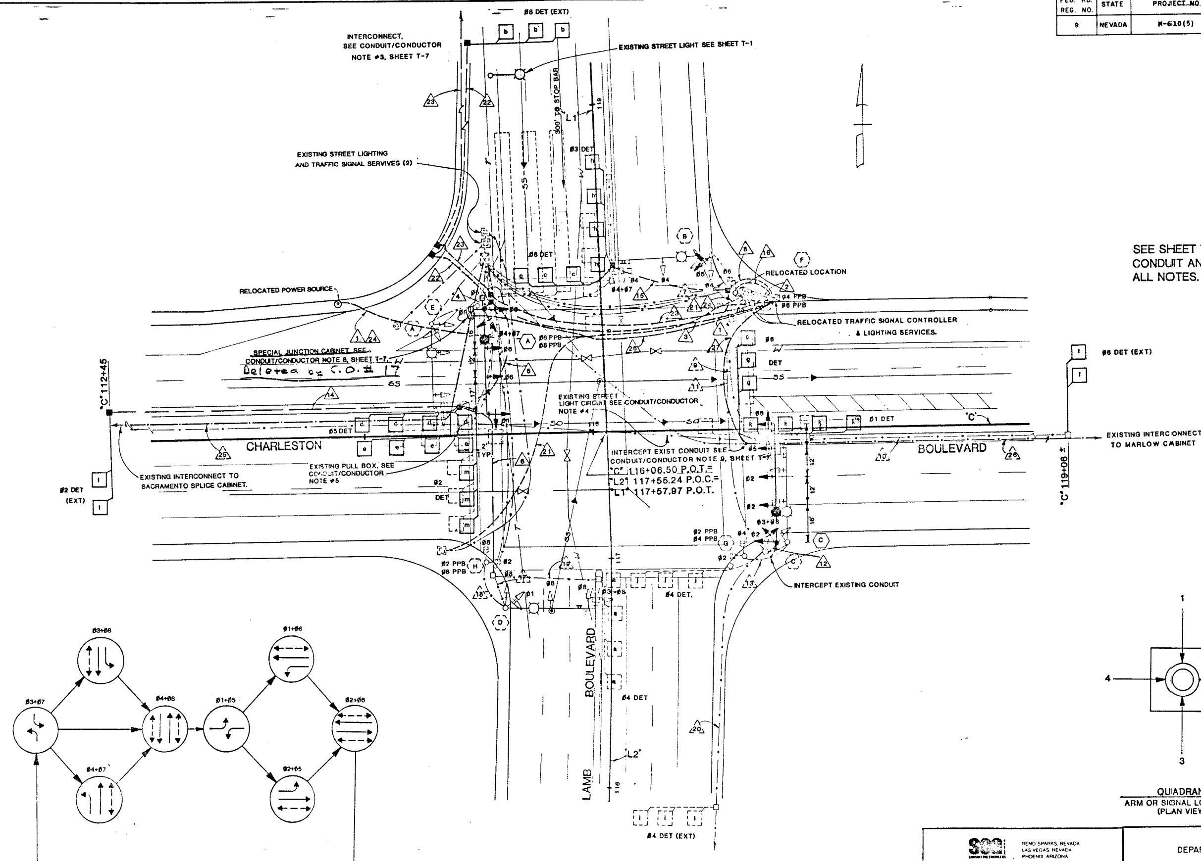
EXISTING PHASING
