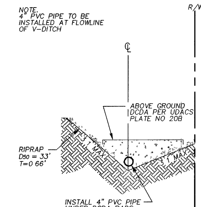
SECTION NTS
