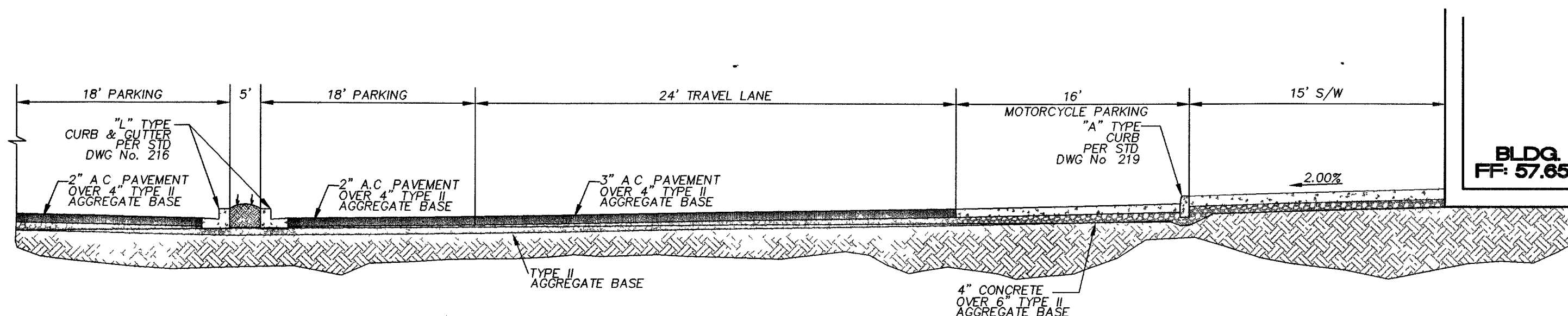
SECTION NTS
