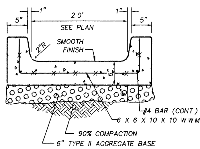
A ON-SITE FLUME NTS
