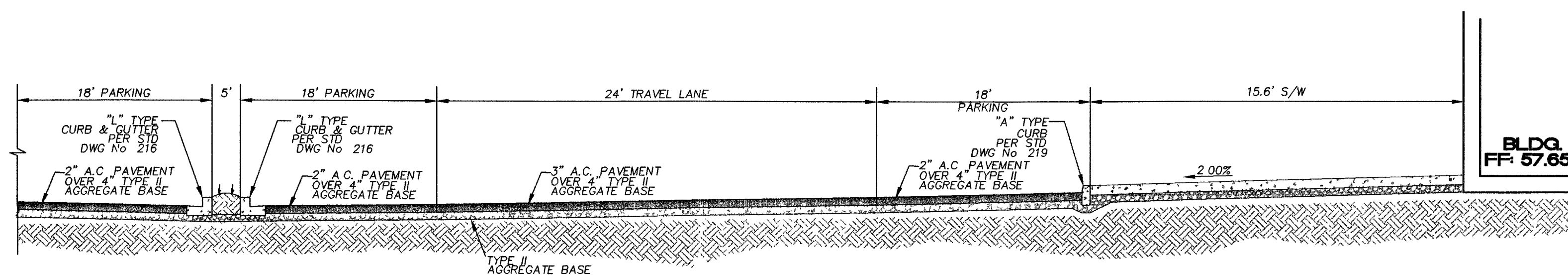
SECTION NTS
