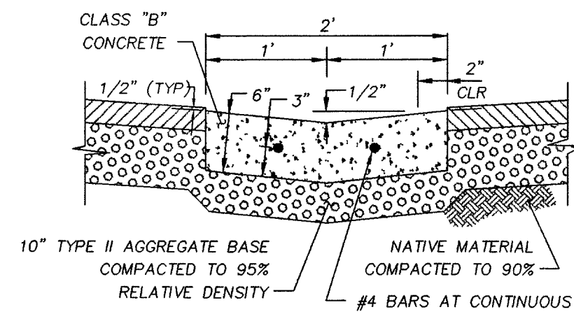
B ON-SITE 2' CONCRETE VALLEY GUTTER NTS
