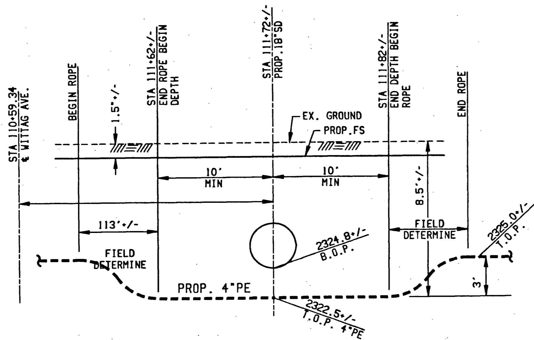
DETAIL "F" SLACK LOWER - N/O WITTIG AVE. VIEW TO WEST NTS
