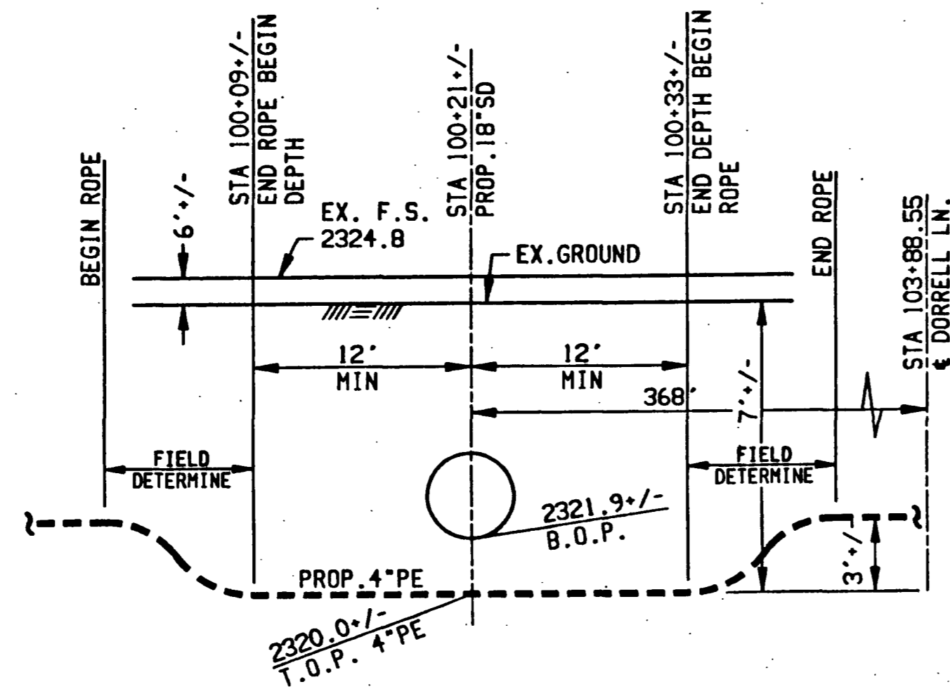
DETAIL "E" SLACK LOWER - S/O DORRELL LN. VIEW TO WEST NTS
