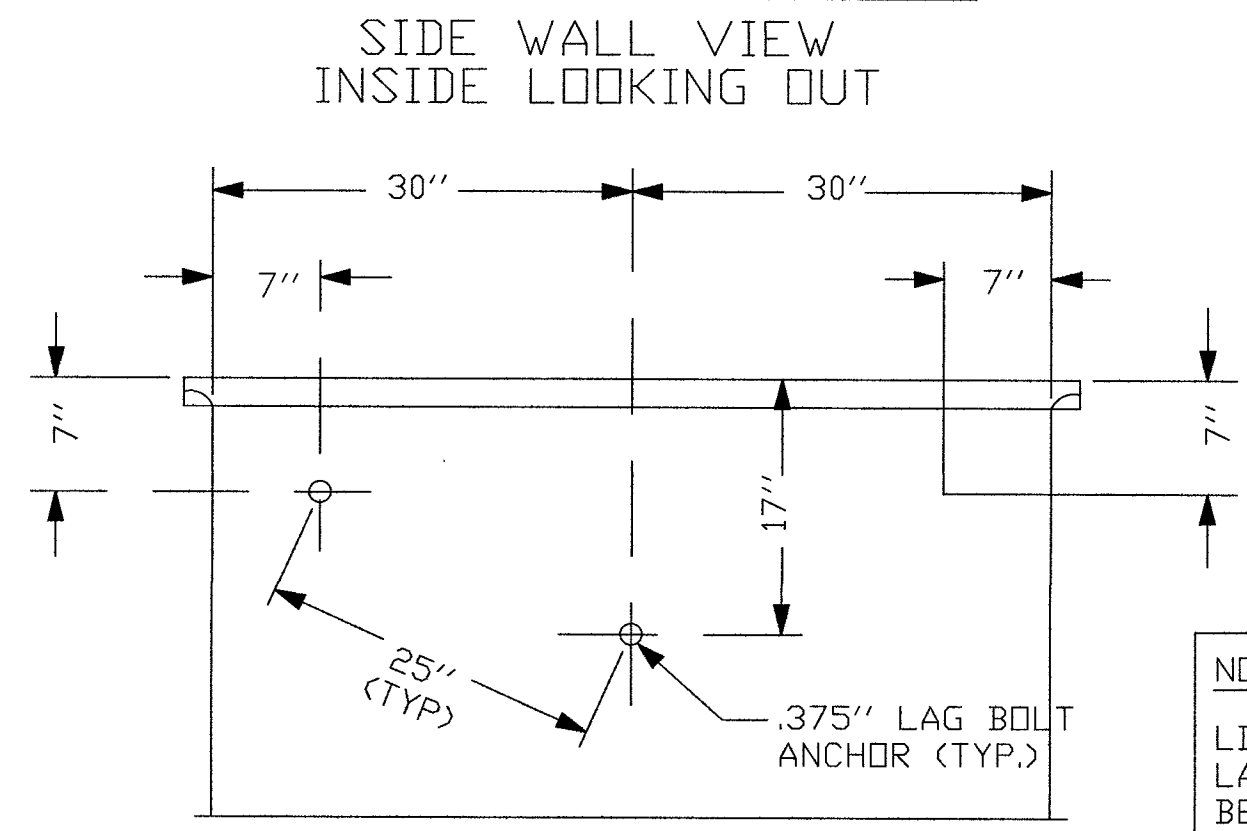
DETAIL "D"
