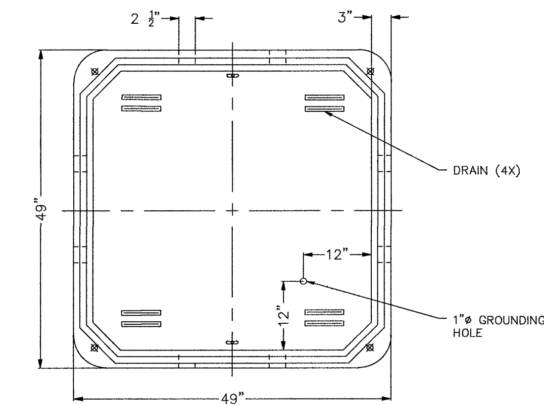
POLYMER CONCRETE MANHOLE TOP VIEW
