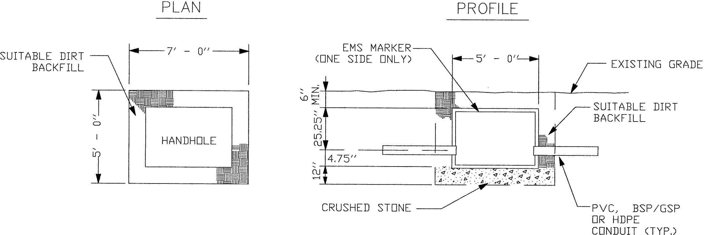
EXCAVATION PIT
