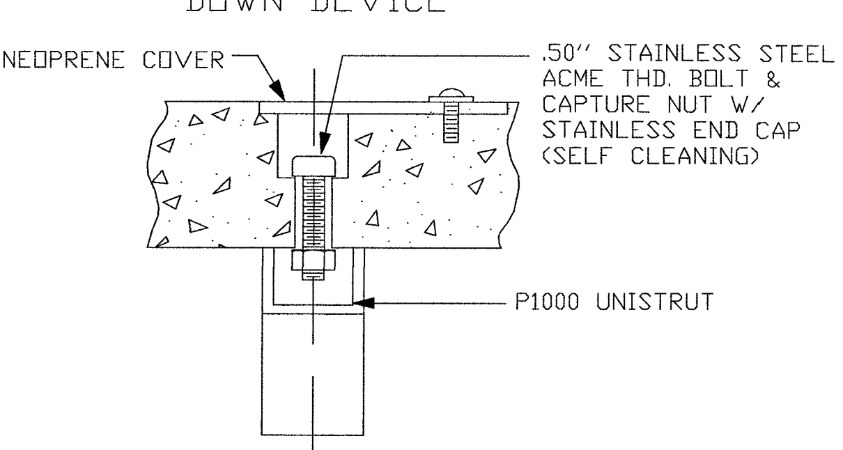
DETAIL "A-3"
