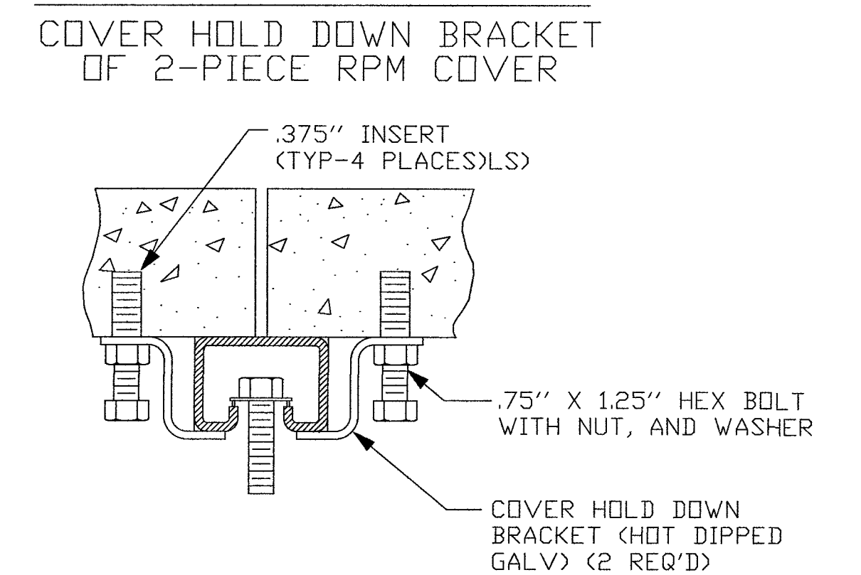
DETAIL "A-4"
