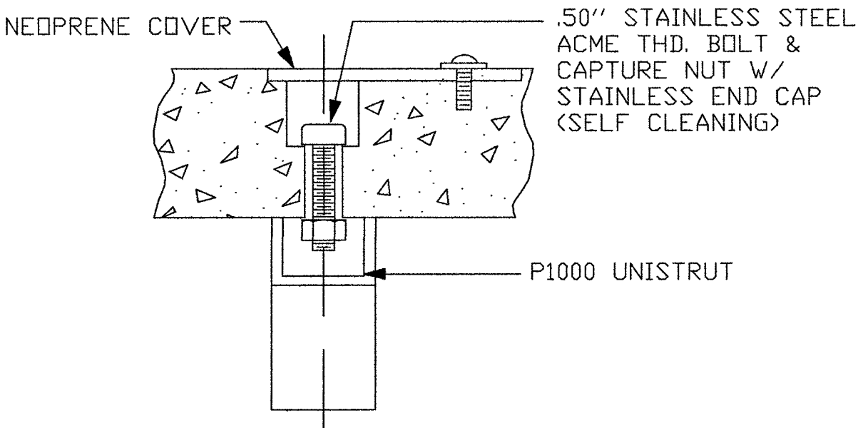
DETAIL "A-3"
