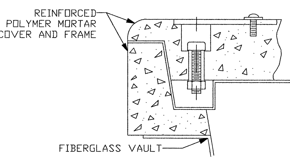
SECTION A-A LOCKING DEVICE CROSS SECTION
