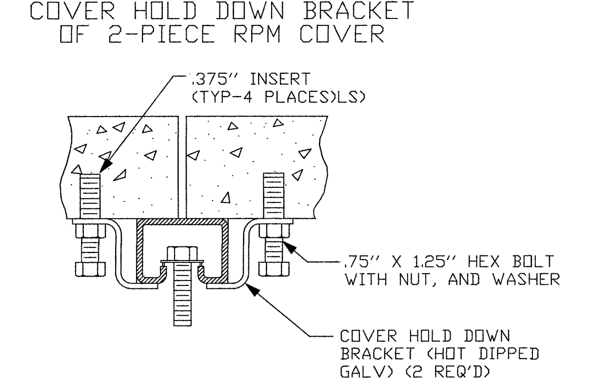
DETAIL "A-4"
