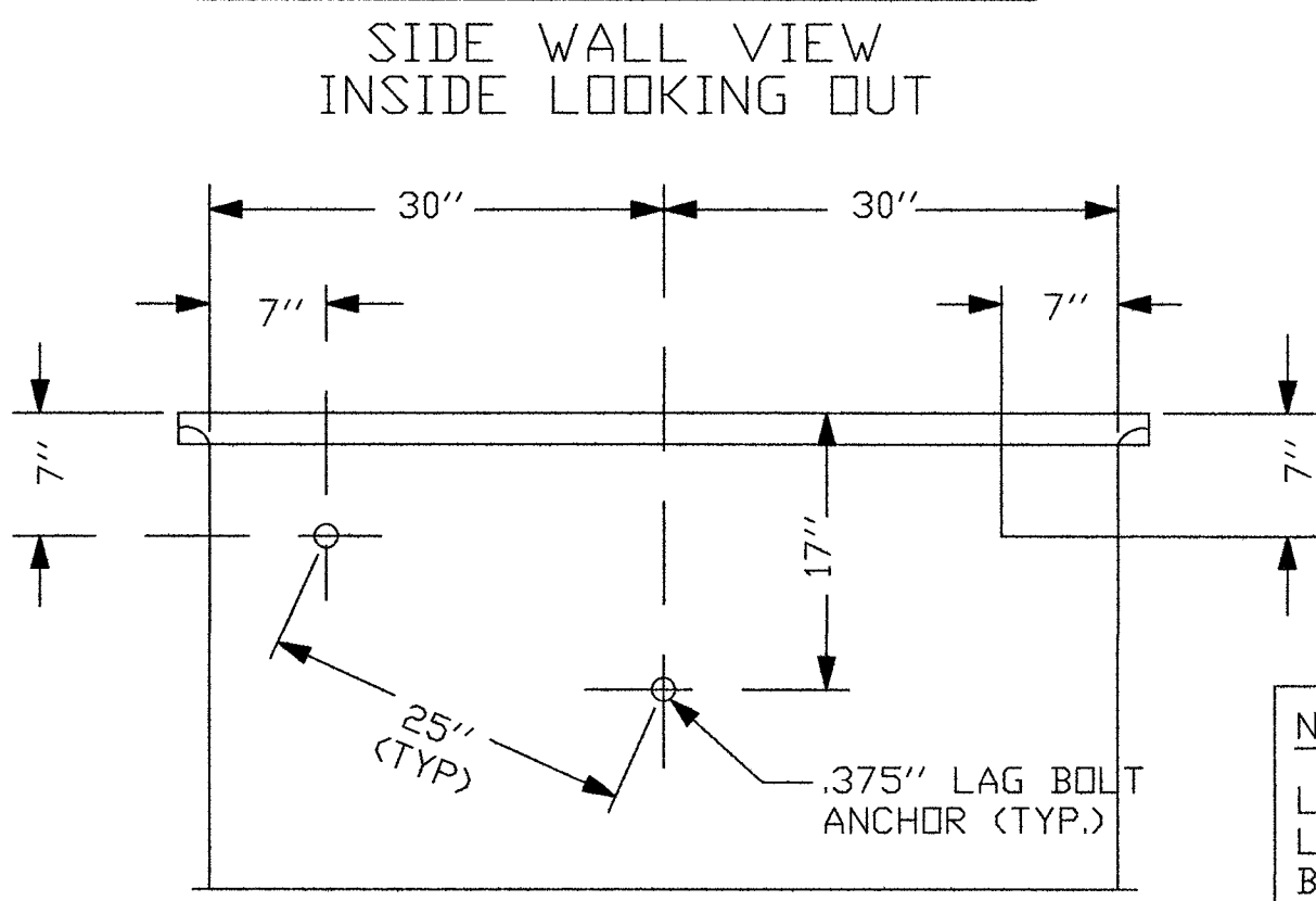
DETAIL "D"
