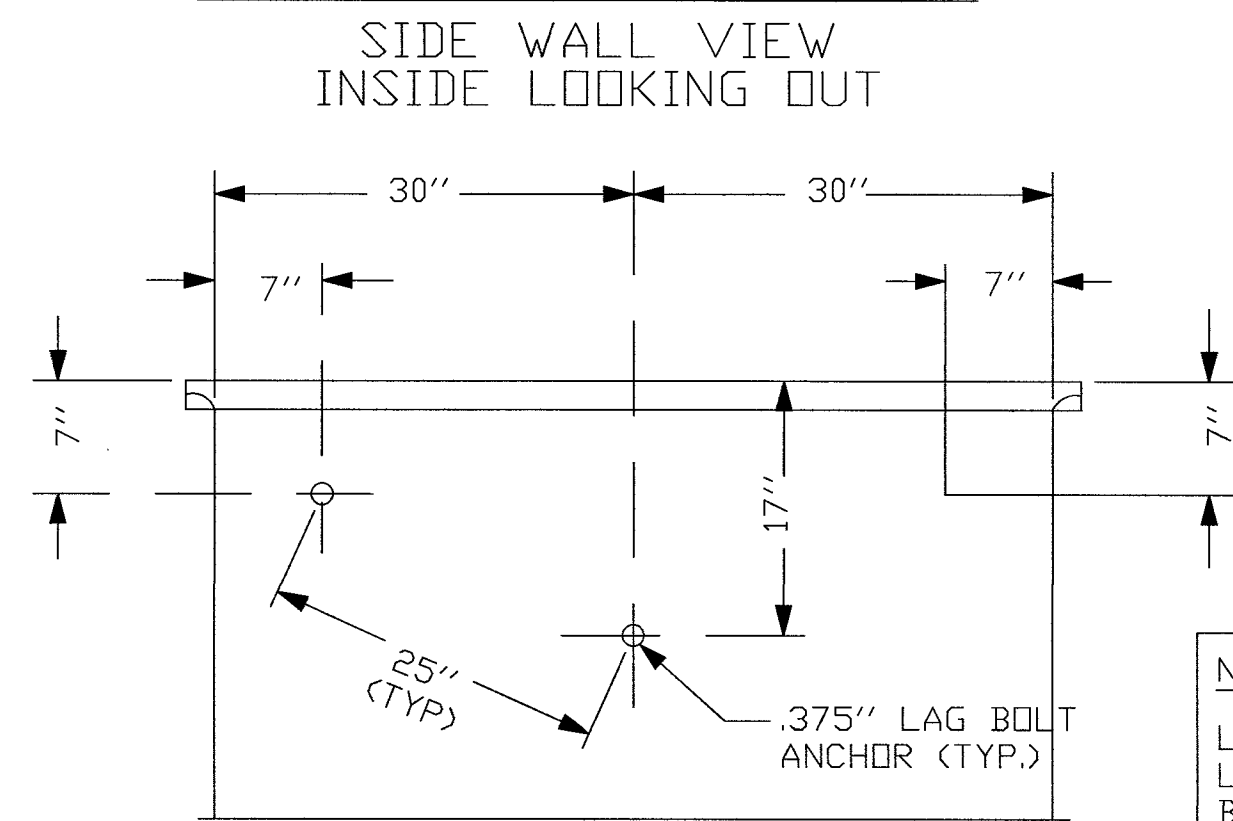
DETAIL "D"
