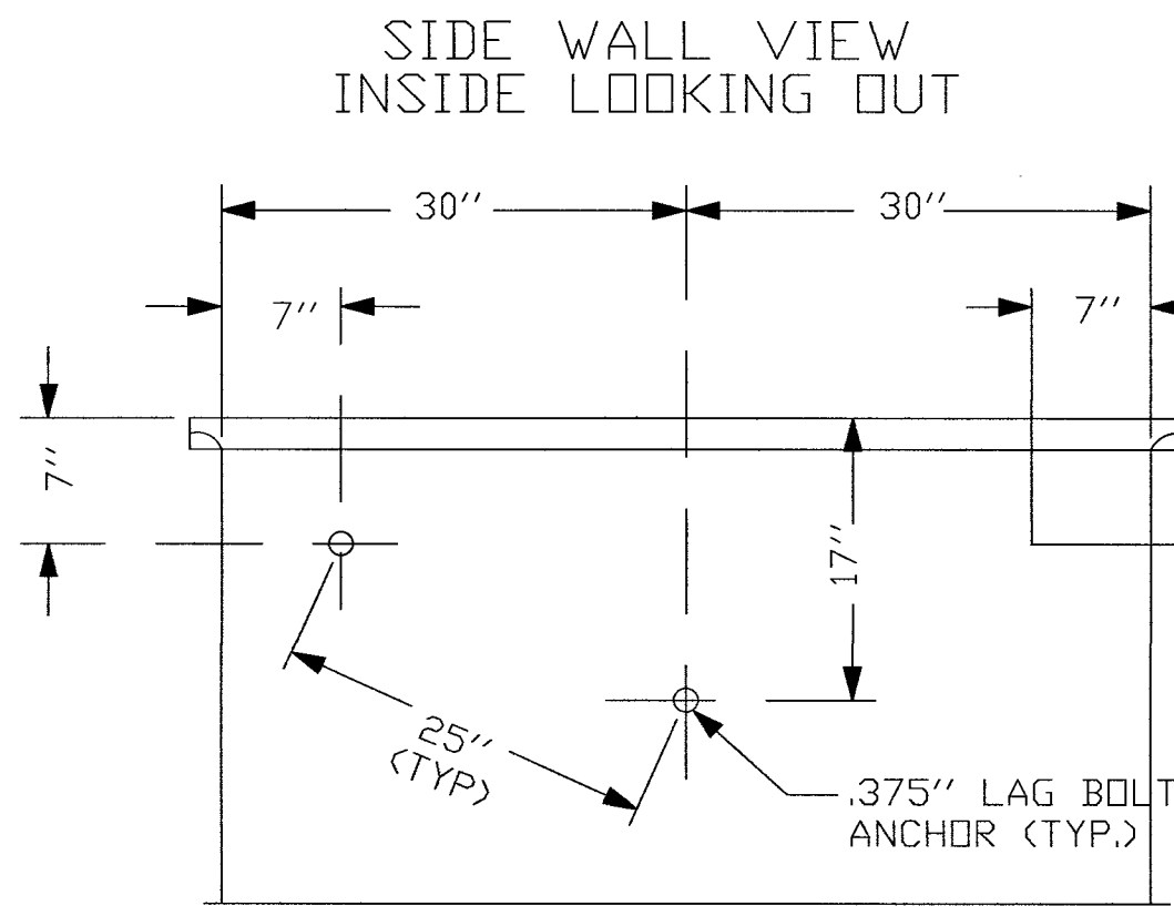
DETAIL "D"
