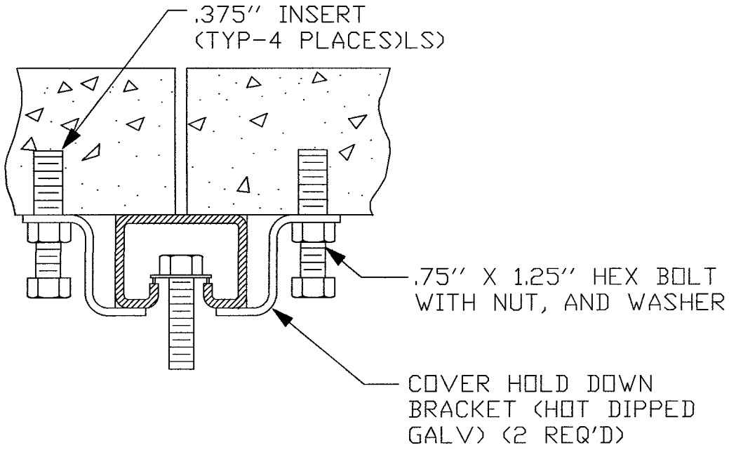
DETAIL "A-4"
