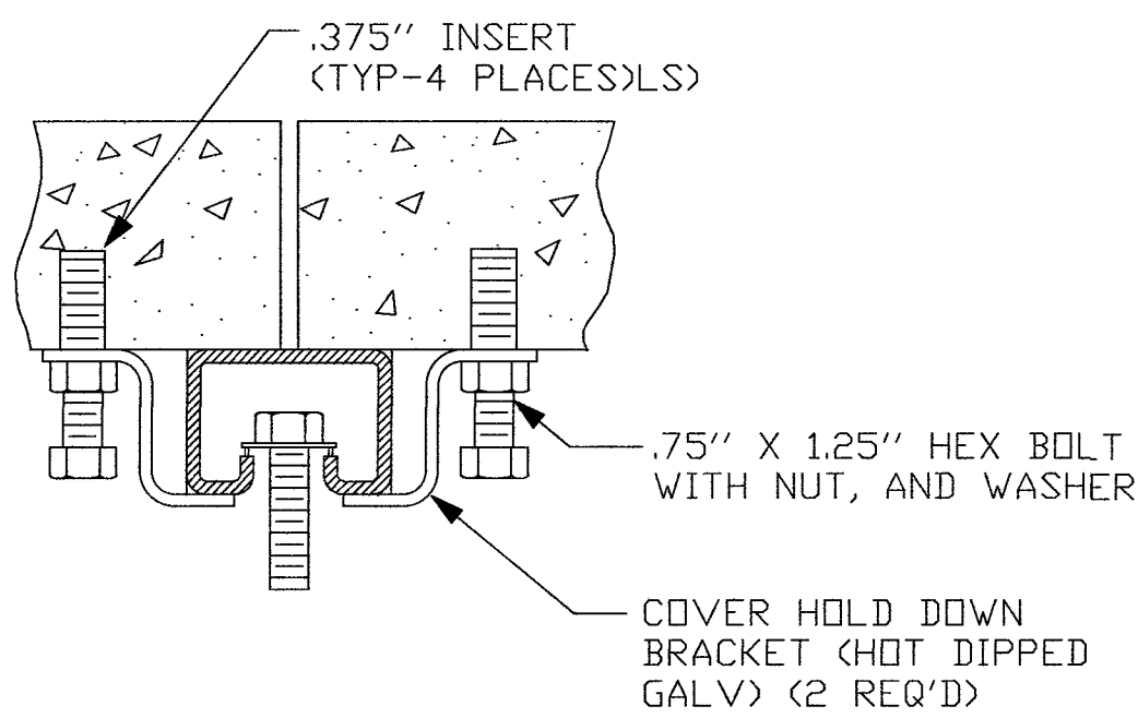
DETAIL "A-4" SUPPORT BEAM INSTALLATION
