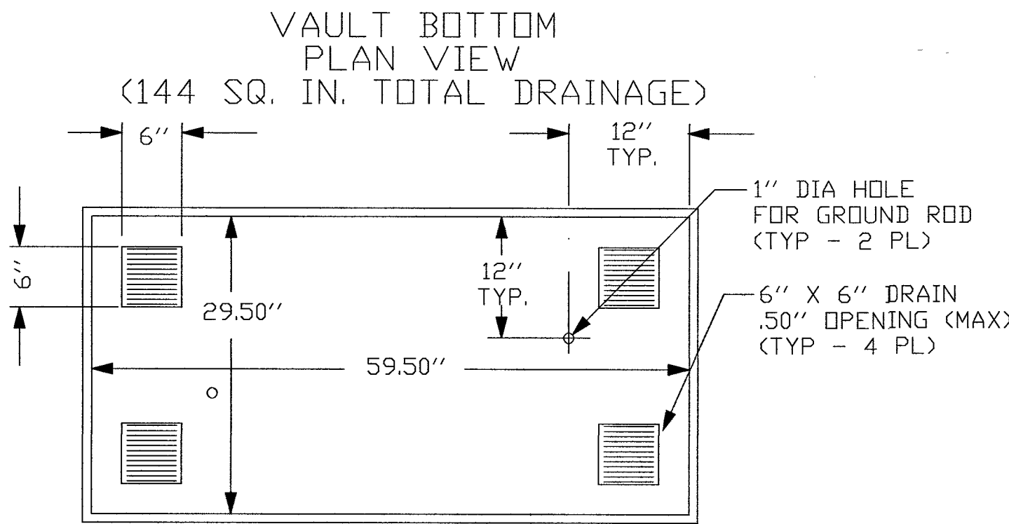
DETAIL "B" VAULT BOTTOM PLAN VIEW
