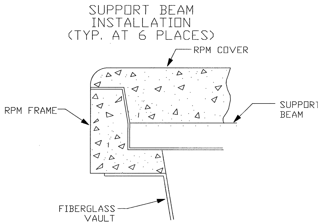
DETAIL "A-4" SUPPORT BEAM INSTALLATION
