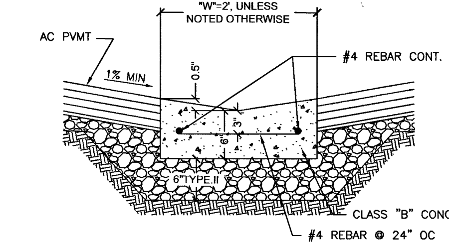
7 VALLEY GUTTER (ON-SITE ONLY) NOT TO SCALE
