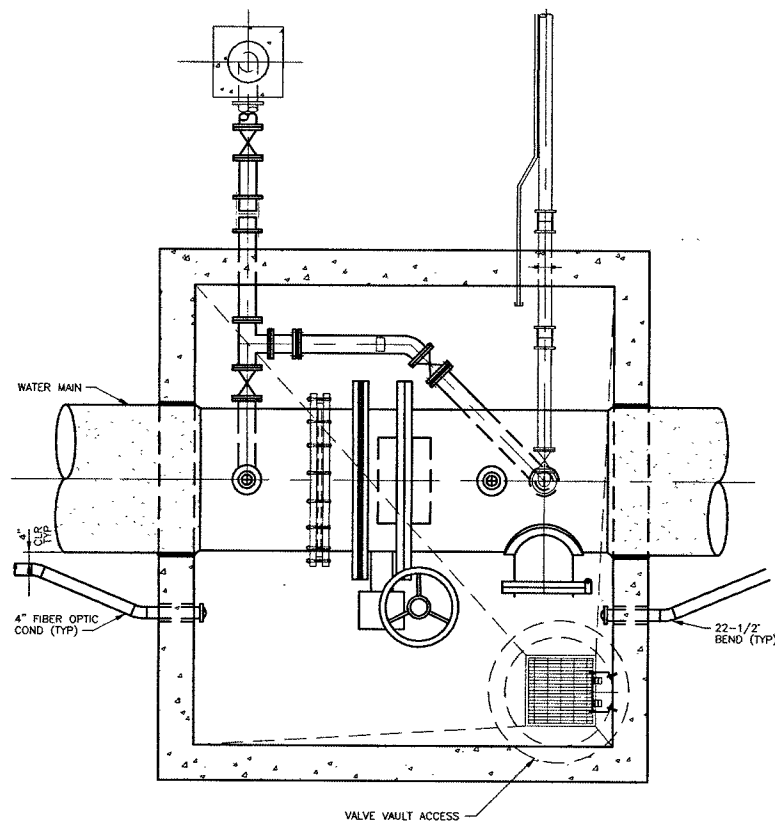
CASE A NOTE: FIBER OPTIC CONDUITS FOUND ON SAME SIDE OF WATER MAIN AS VALVE VAULT ACCESS
