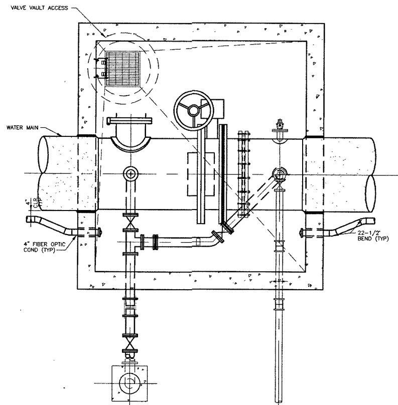
CASE B NOTE: FIBER OPTIC CONDUITS FOUND ON OPPOSITE SIDE OF WATER MAIN AS VALVE VAULT ACCESS
