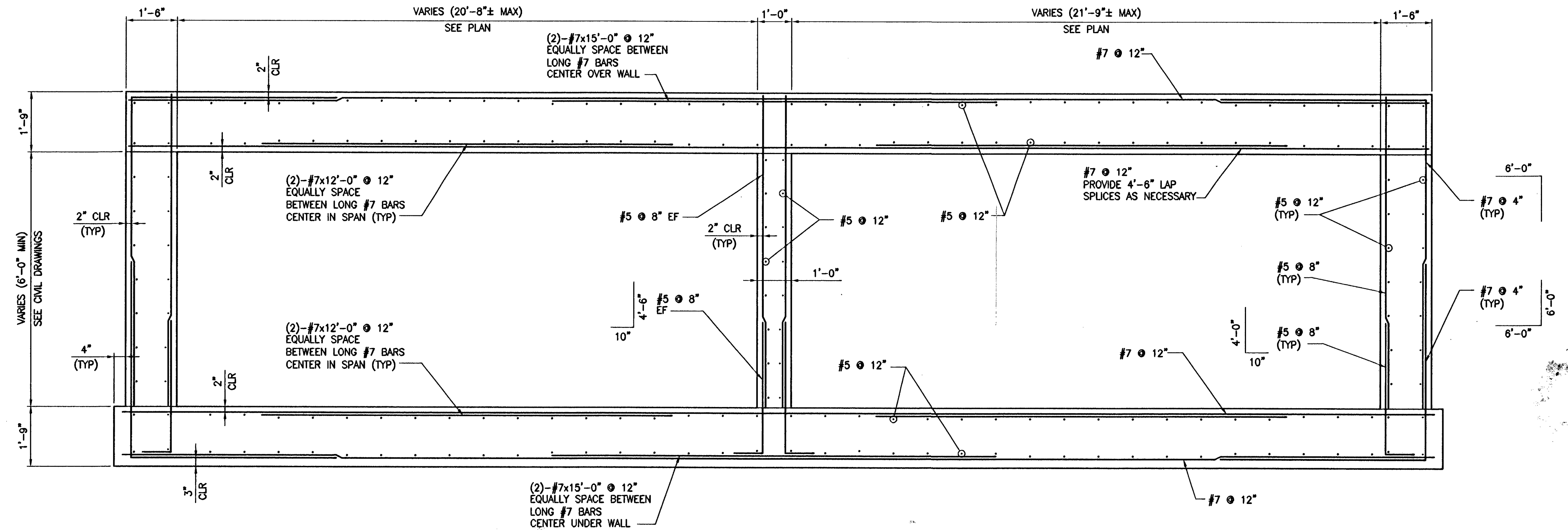
B SECTION
