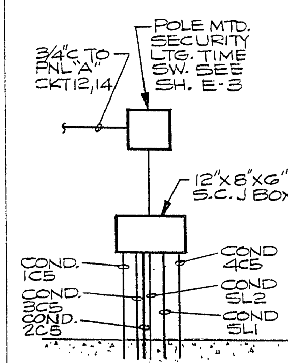
ELEVATION F NO SCALE
