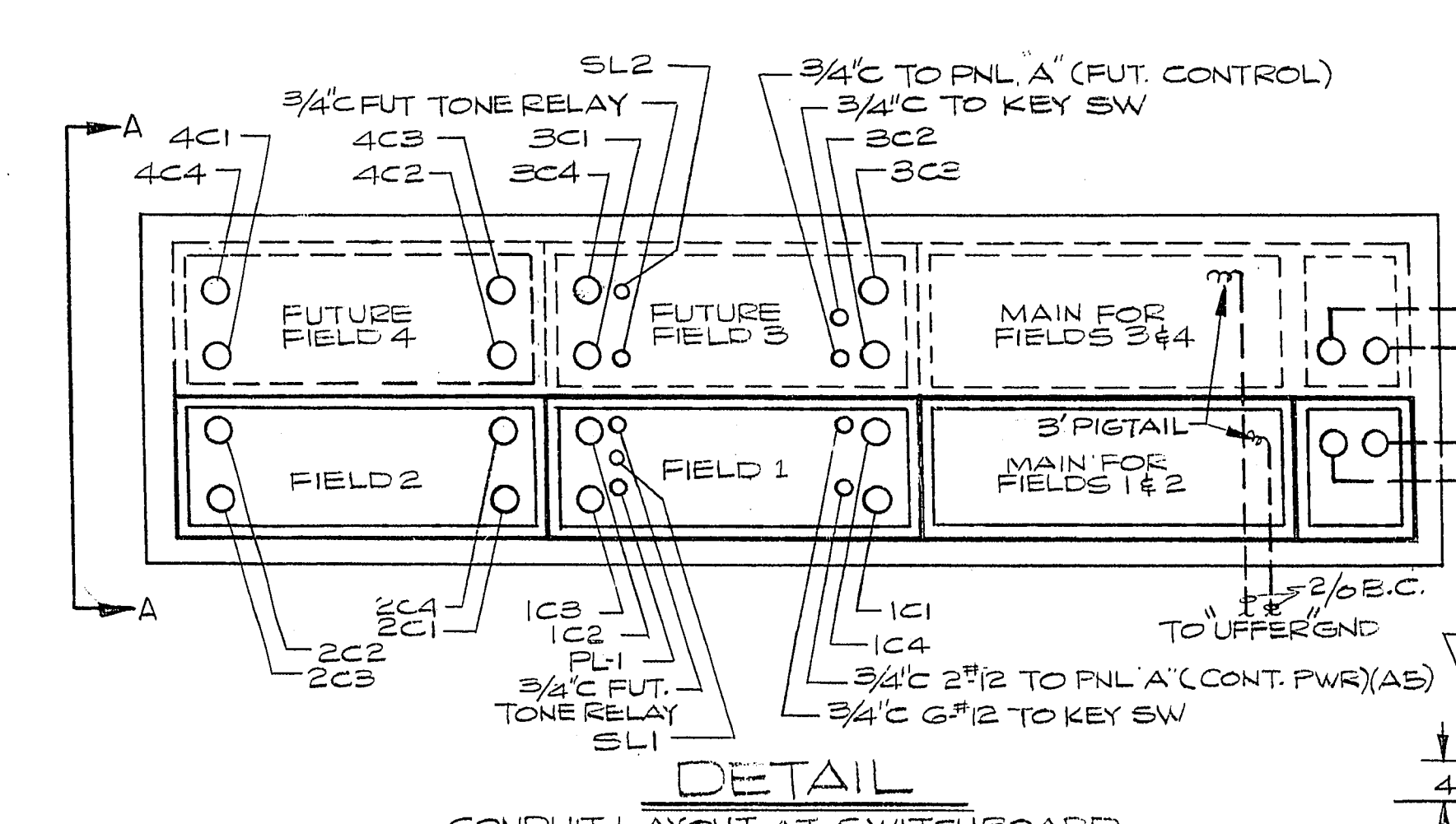
DETAIL CONDUIT LAYOUT AT SWITCHBOARD NO SCALE NOTE: ALL CONDUIT TO BE INSTALLED IN THIS PHASE
