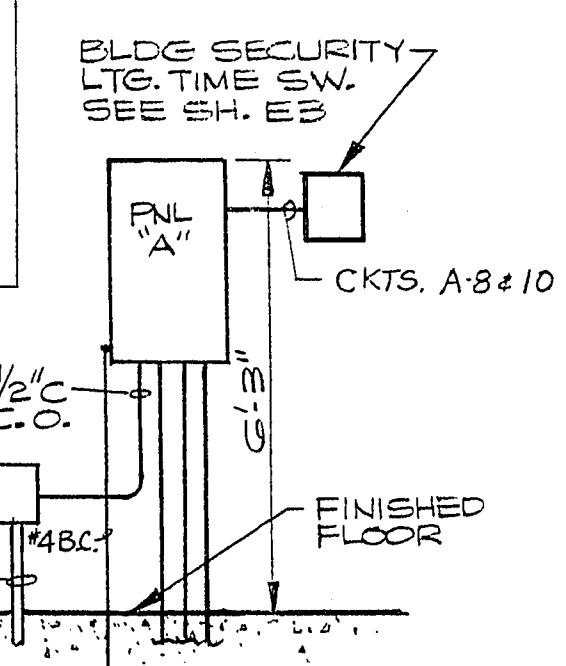
ELEVATION B NO SCALE
