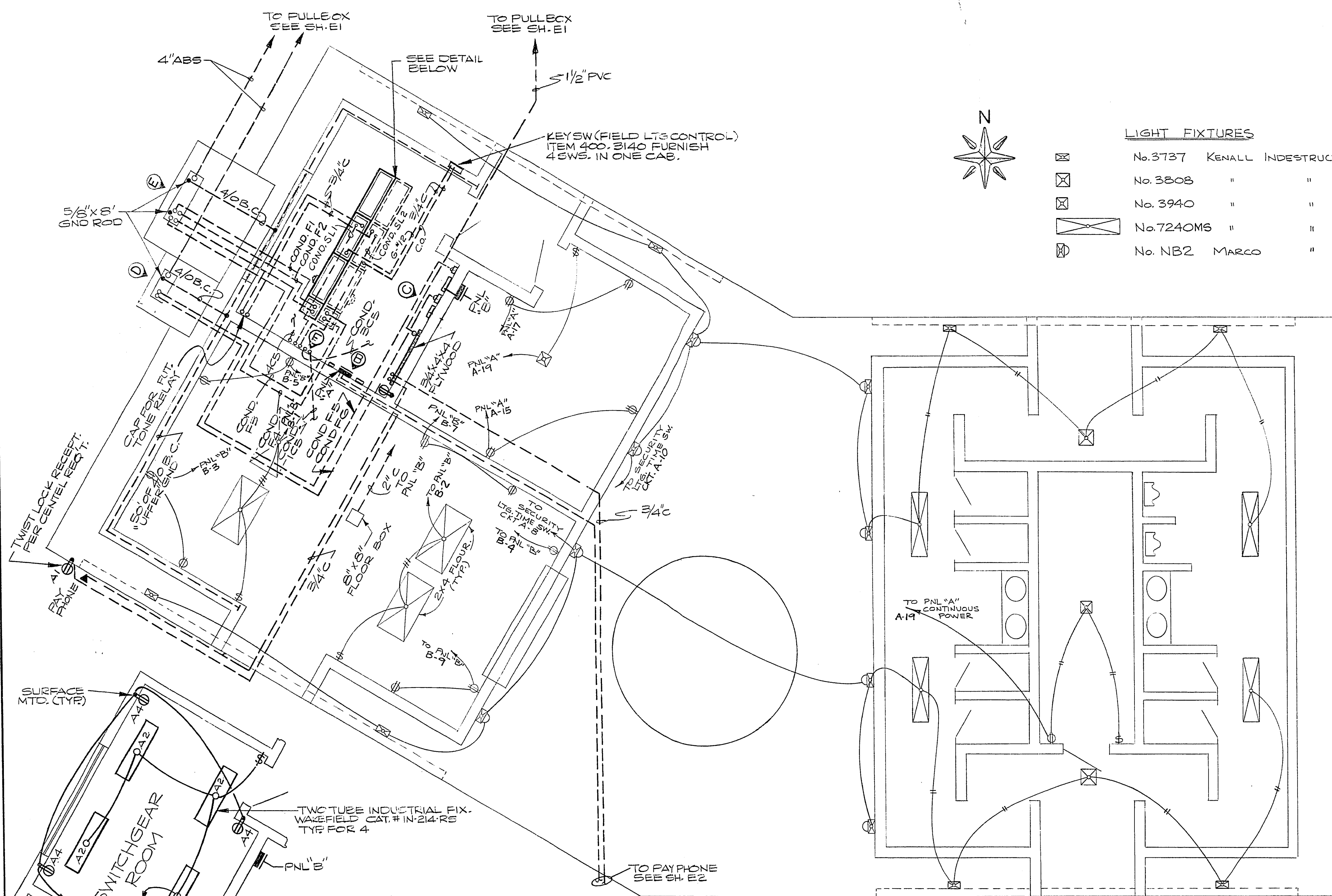
PARTIAL LIGHTING PLAN SCALE 1/4"=1'-0"
