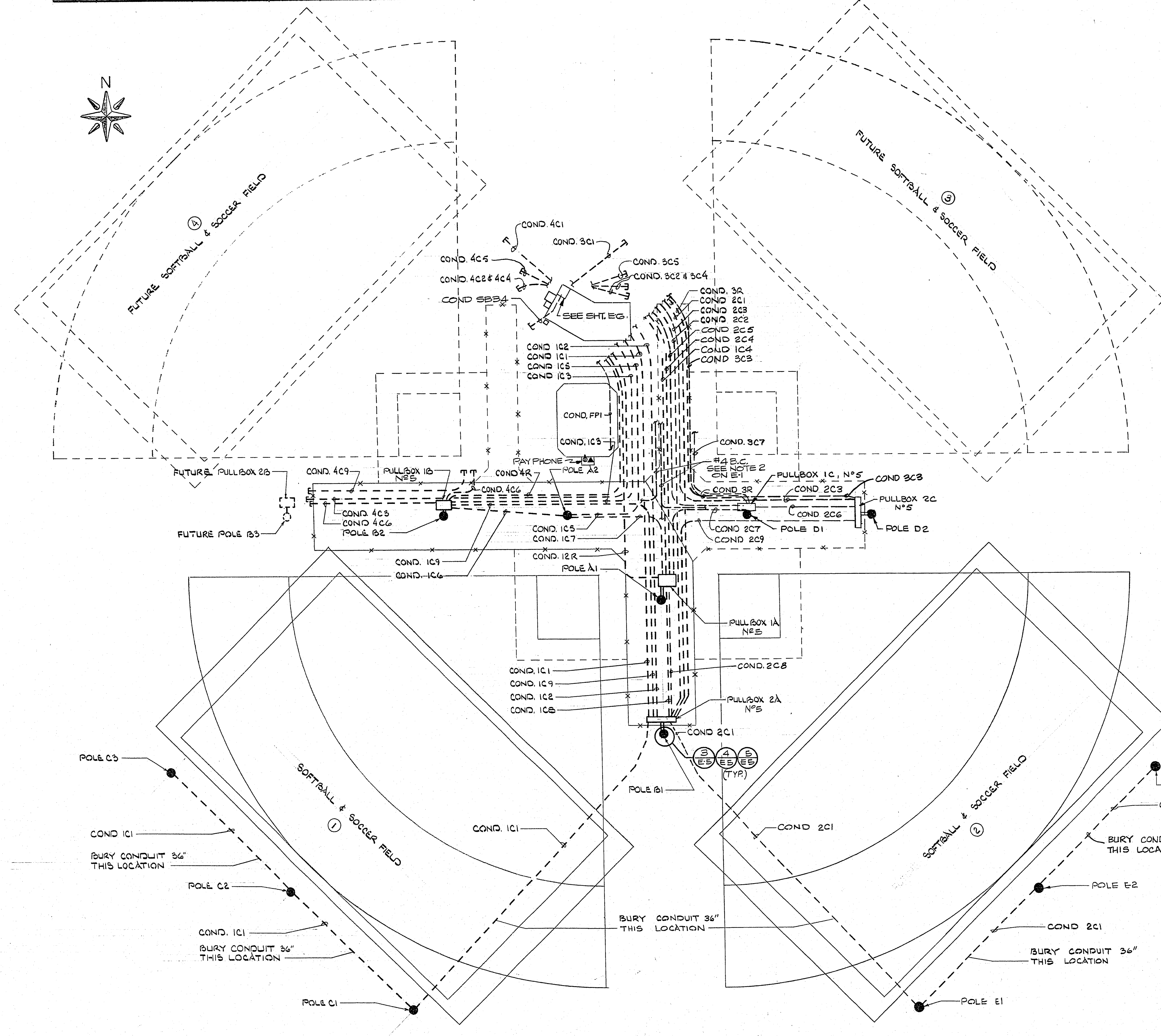
ENLARGED PLAN OF FIELD AREA SCALE=1"=50'
