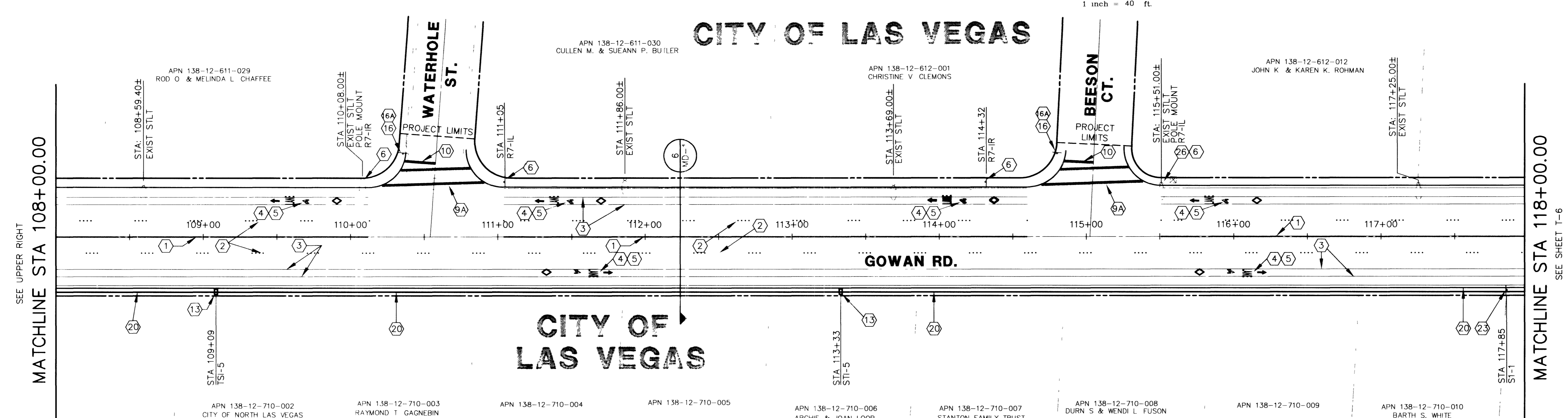
PLAN - GOWAN ROAD
