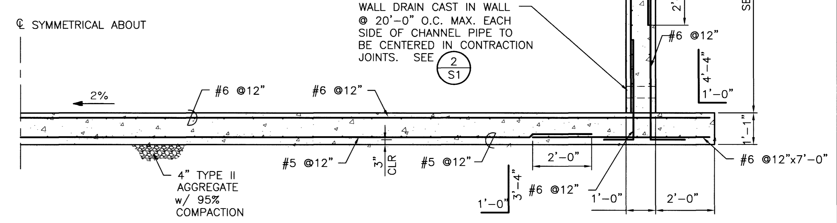
ABUTMENT SECTION SCALE: 1/2" = 1'-0" (A S6)
