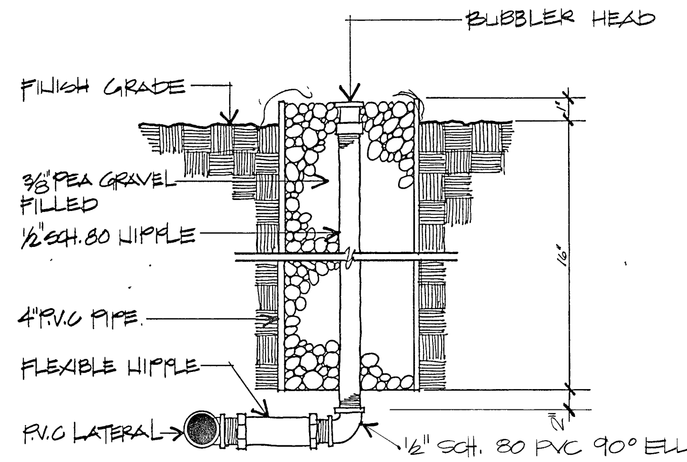
6 TREE BUBBLER DETAIL
