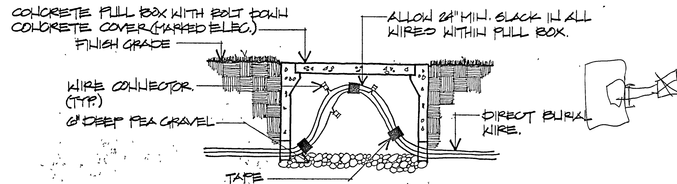
8 24 VOLT WIRE SPLICING DETAIL
