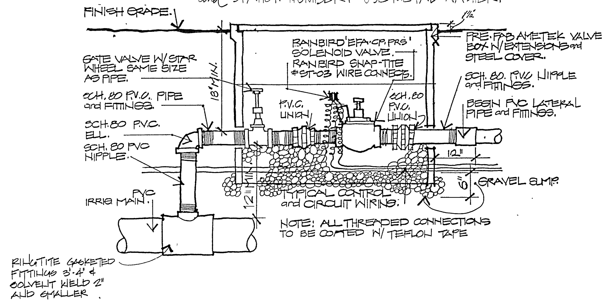
7 TYPICAL LAWN & SHRUB VALVE DETAIL
