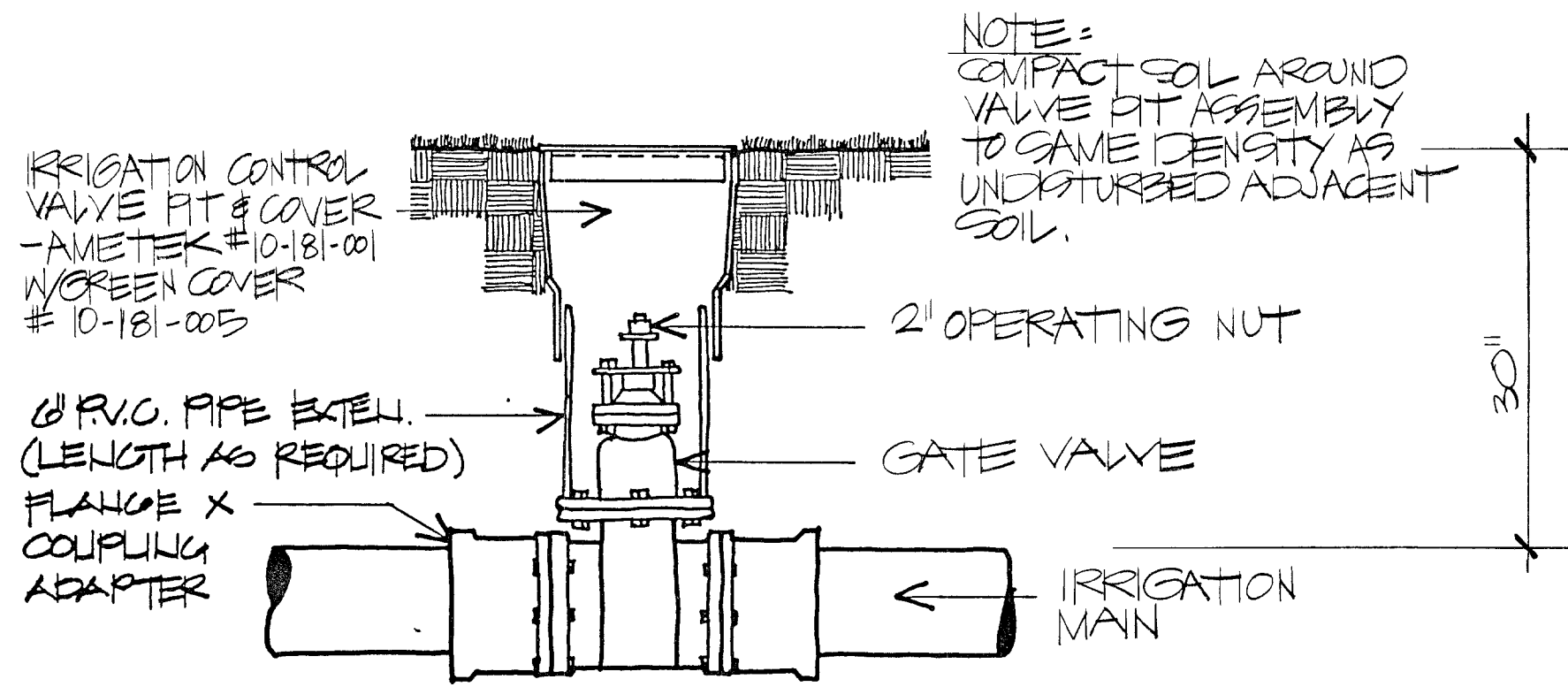
9 GATE VALVE DETAIL
