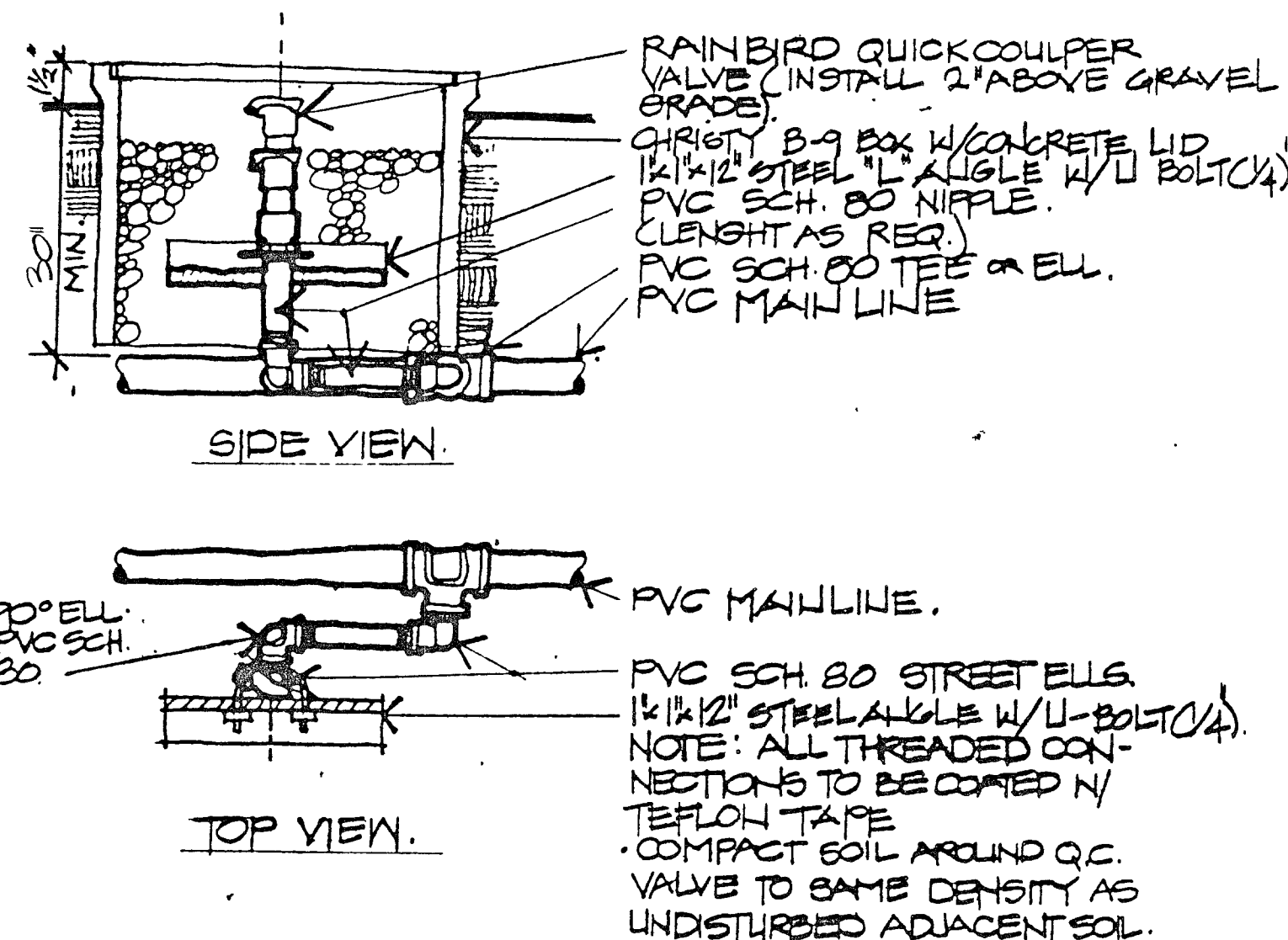
4 QUICK COUPLER DETAIL
