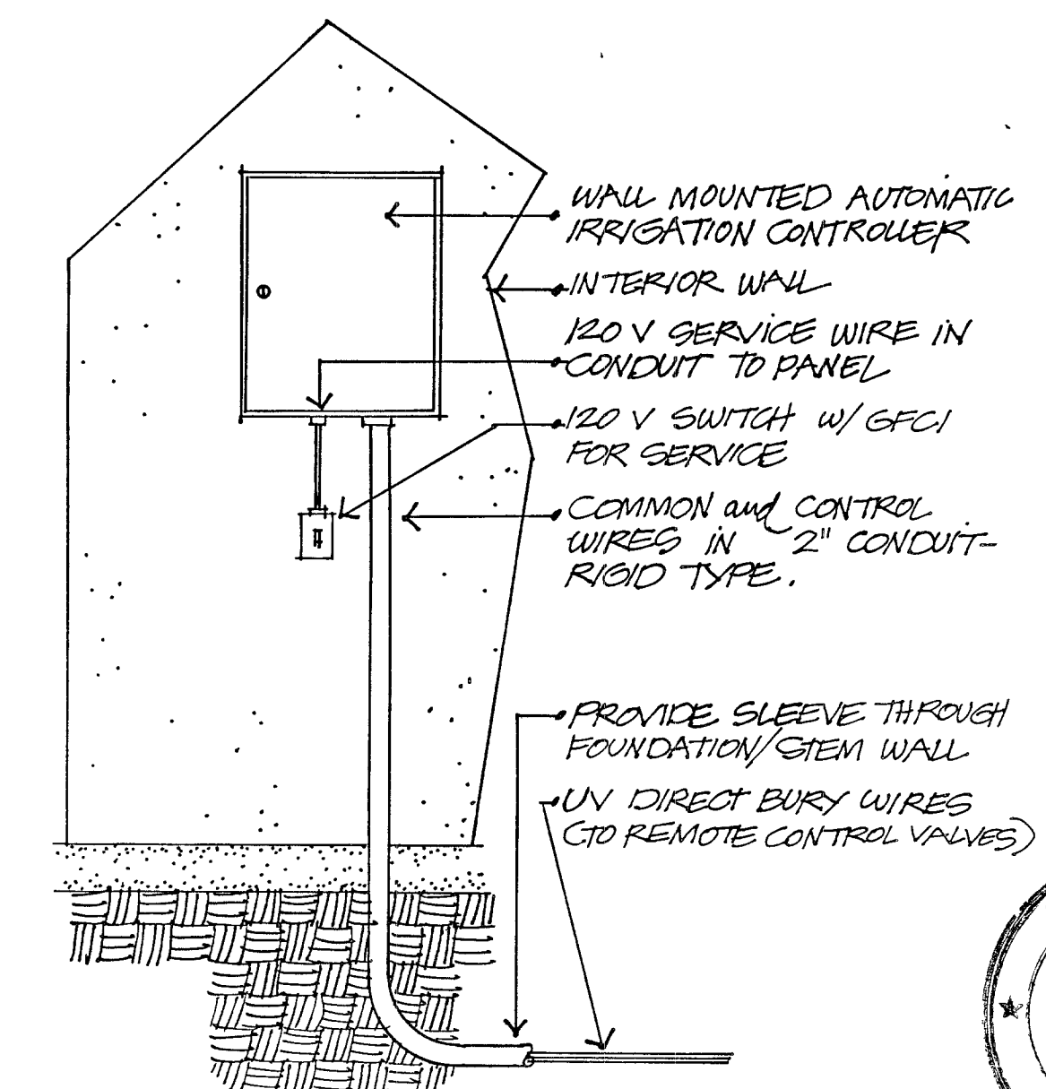
1 WALL MOUNTED IRRIGATION CONTROLLER
