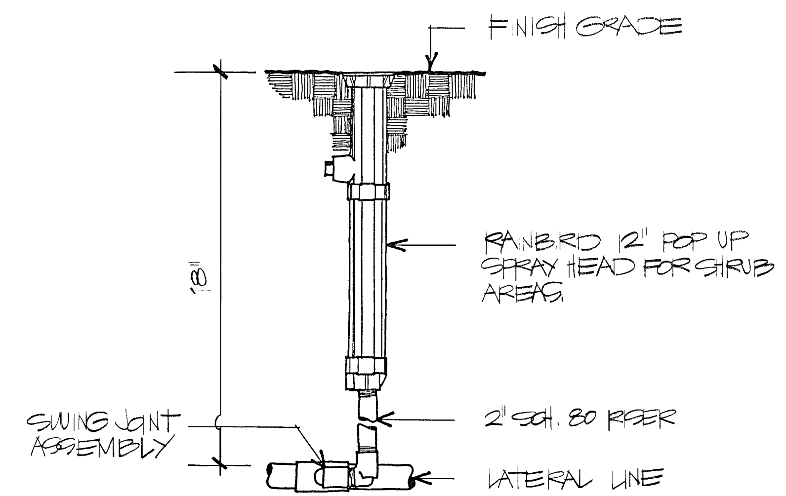
3 12" POP UP SPRAY HEAD (FOR SHRUB AREAS)
