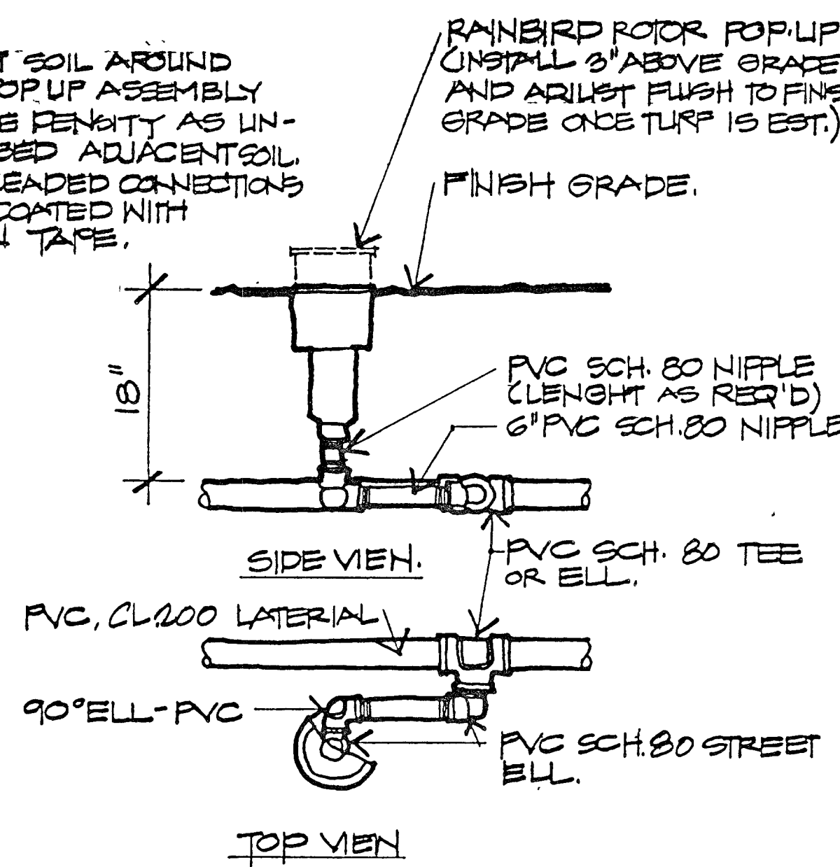
5 ROTOR POP UP DETAIL
