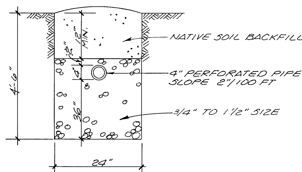
ABSORPTION TRENCH
