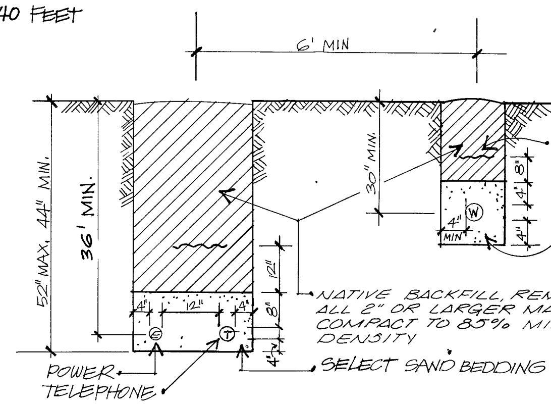
UTILITY TRENCH DETAIL
