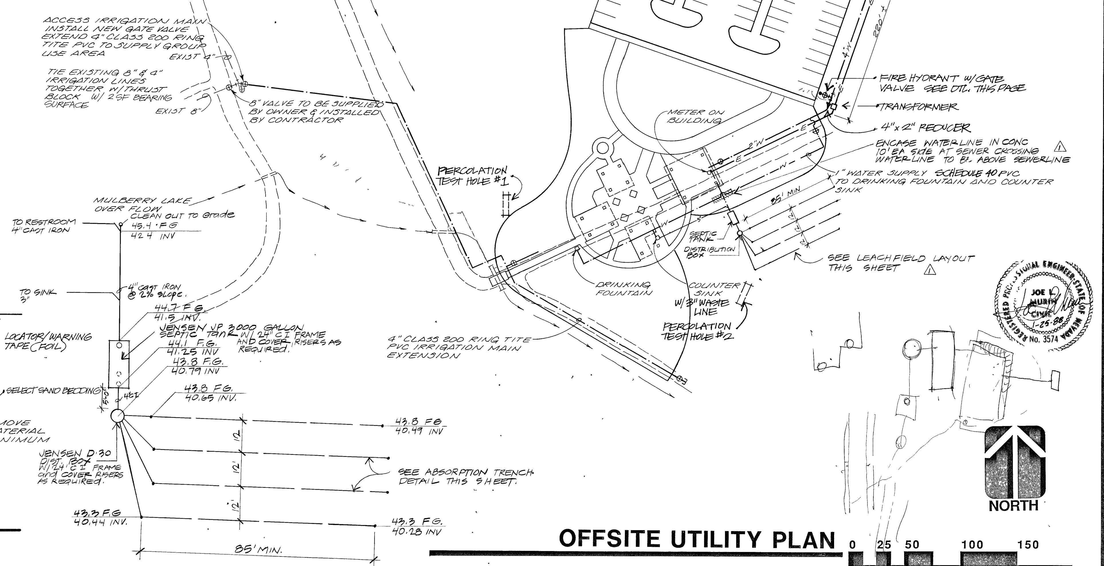
LEACHFIELD LAYOUT
