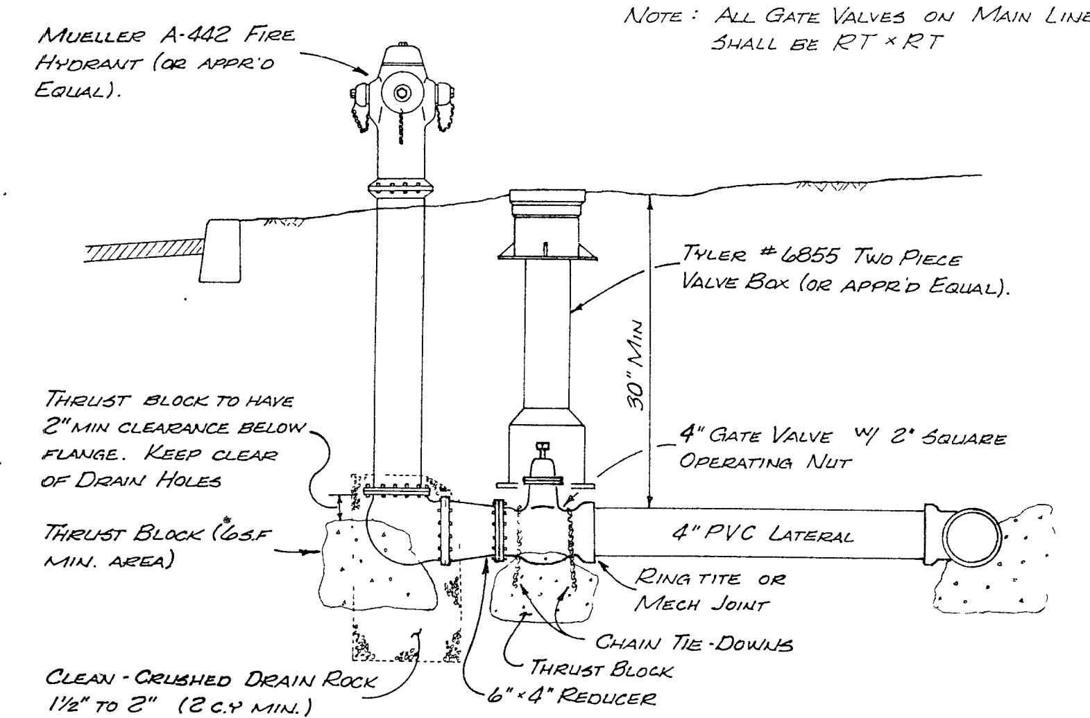
FIRE HYDRANT ASSEMBLY
