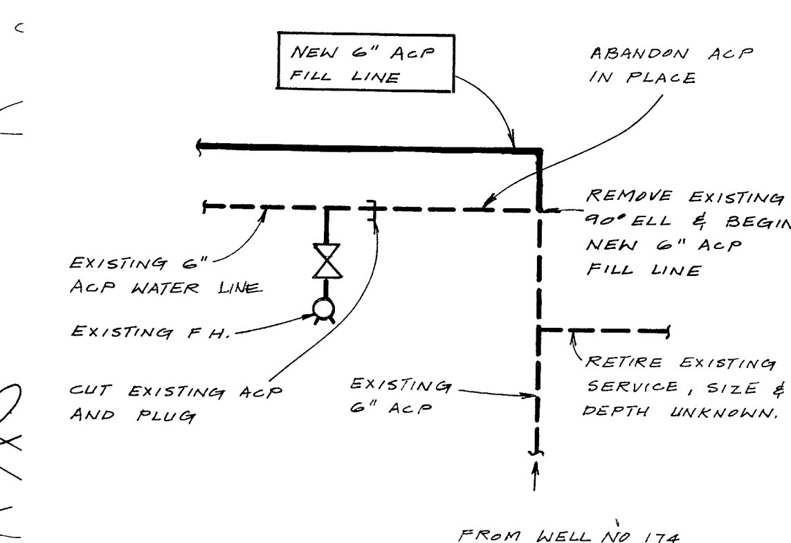
A DETAIL U-1 NTS
