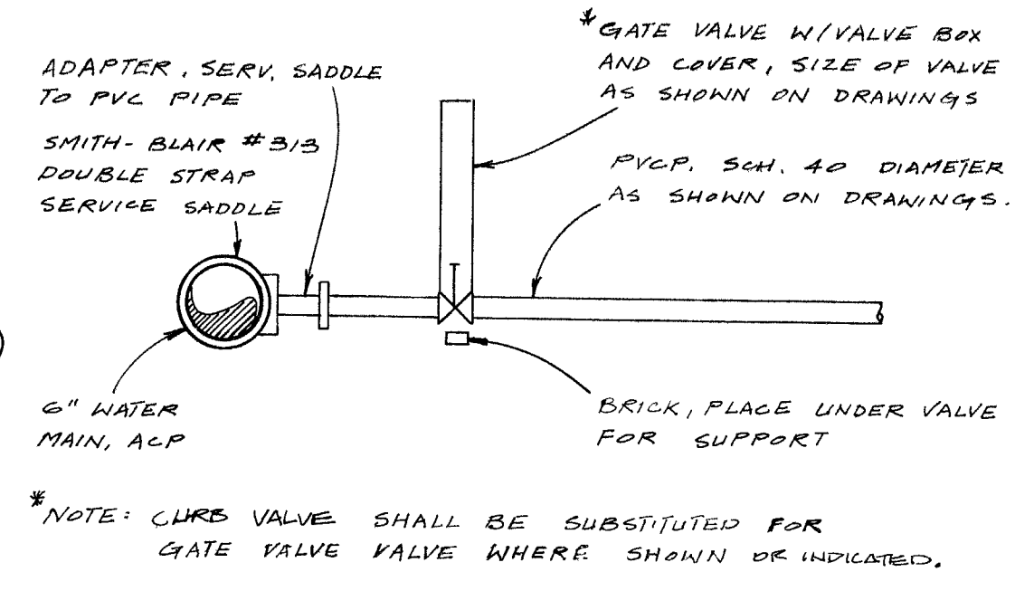
B WATER SERVICE CONNECTION DETAIL U-1 NTS
