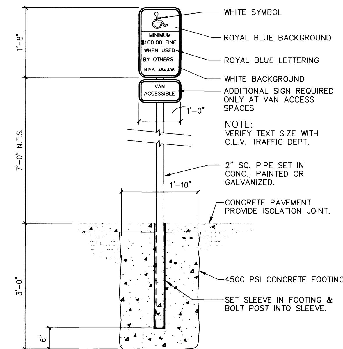
7 Handicap Accessibility Sign Scale: 3/4" = 1'-0" 10426-01 AS2-09
