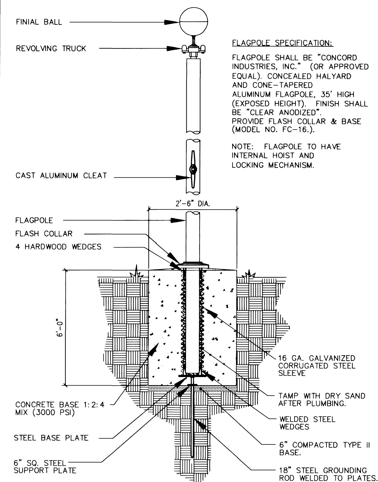
8 Flagpole Base Detail
