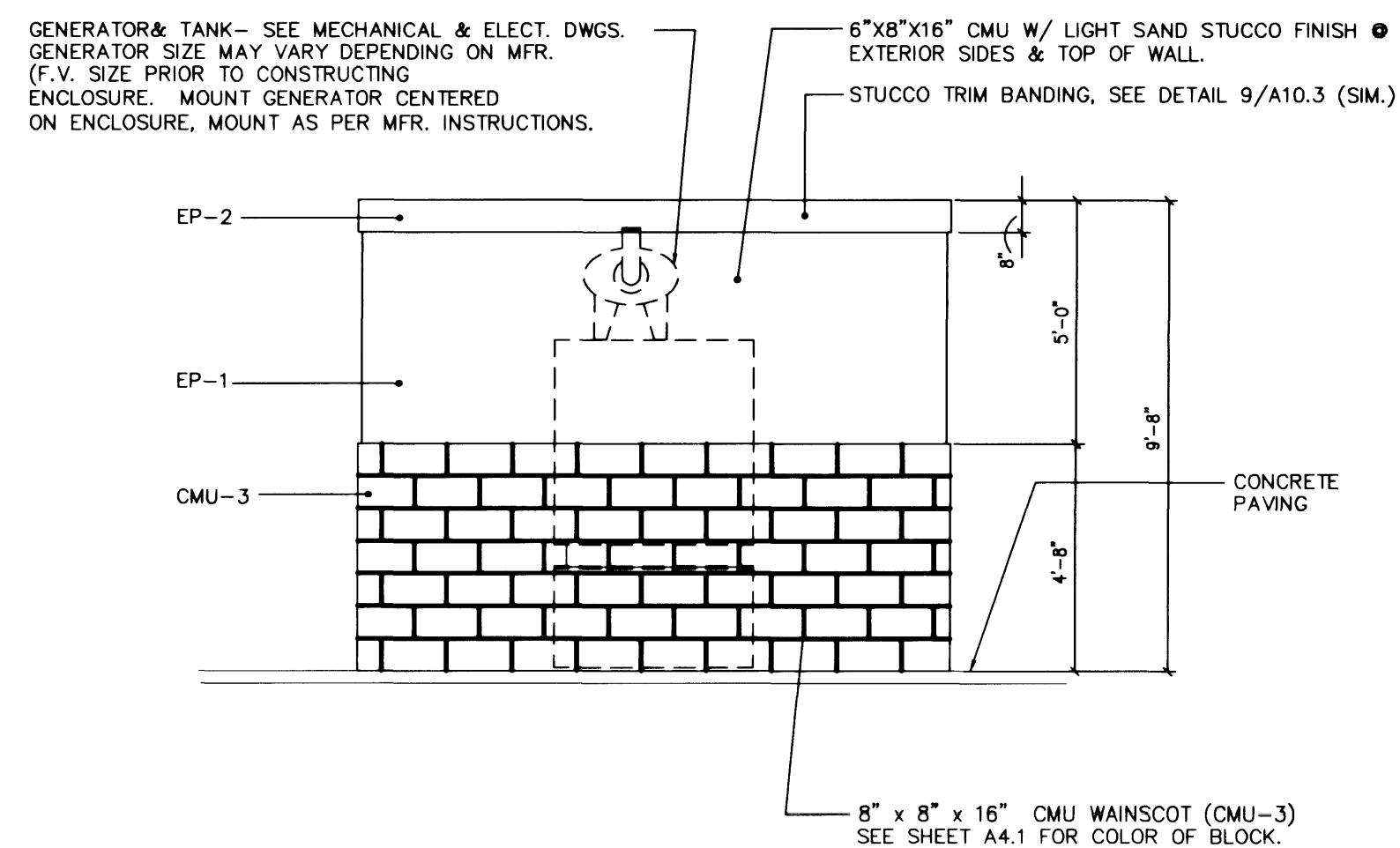
9B Generator Enclosure – East Elevation
