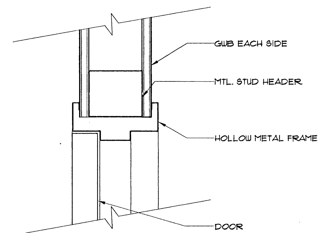
4 Interior Door Head - Jamb Sim. Scale: 3\"/>
