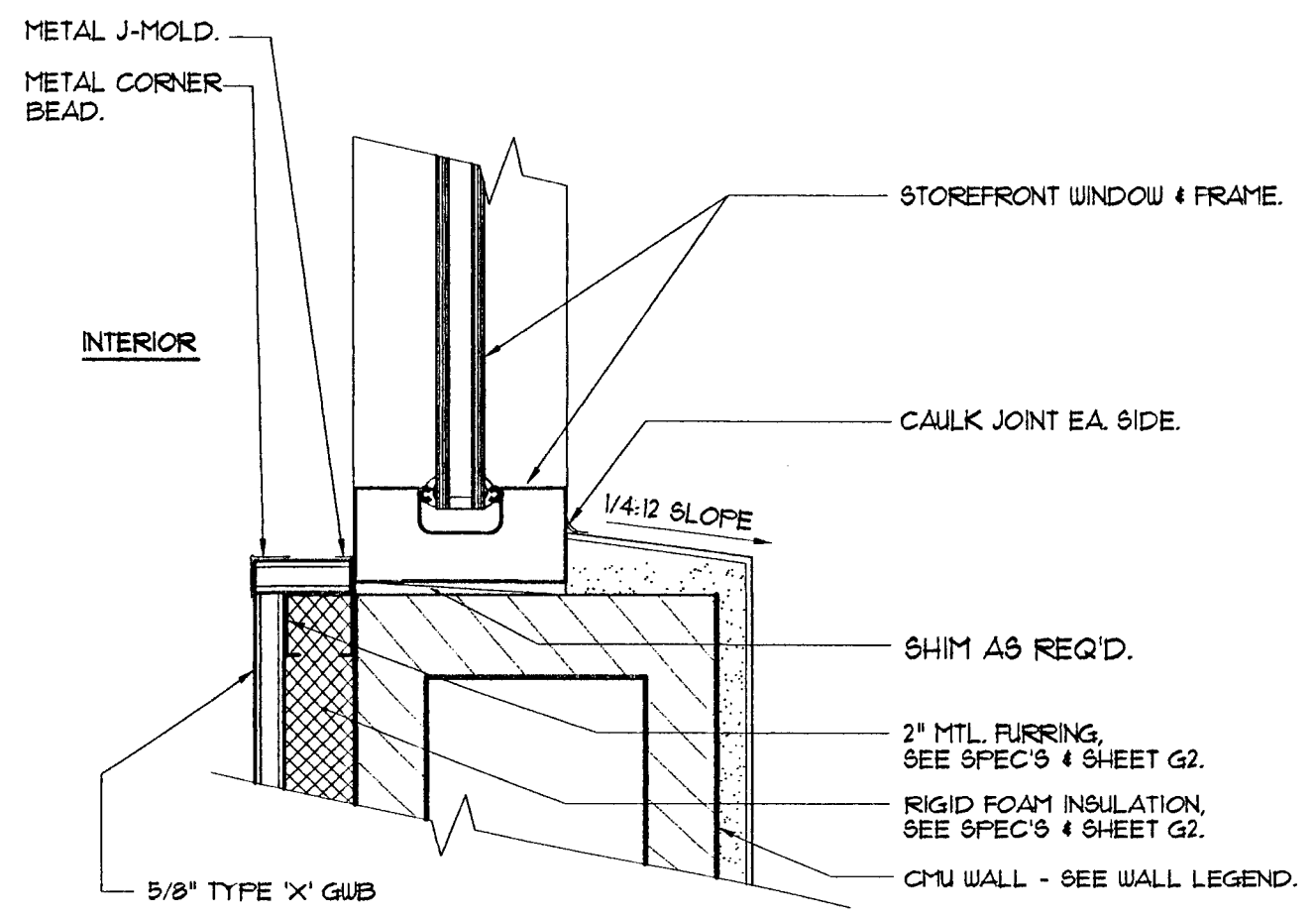
7 Exterior Window Sill Detail Scale: 3\"/>
