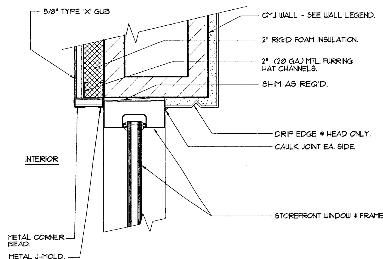
5 Exterior Window Jamb/ Head Detail Scale: 3\"/>
