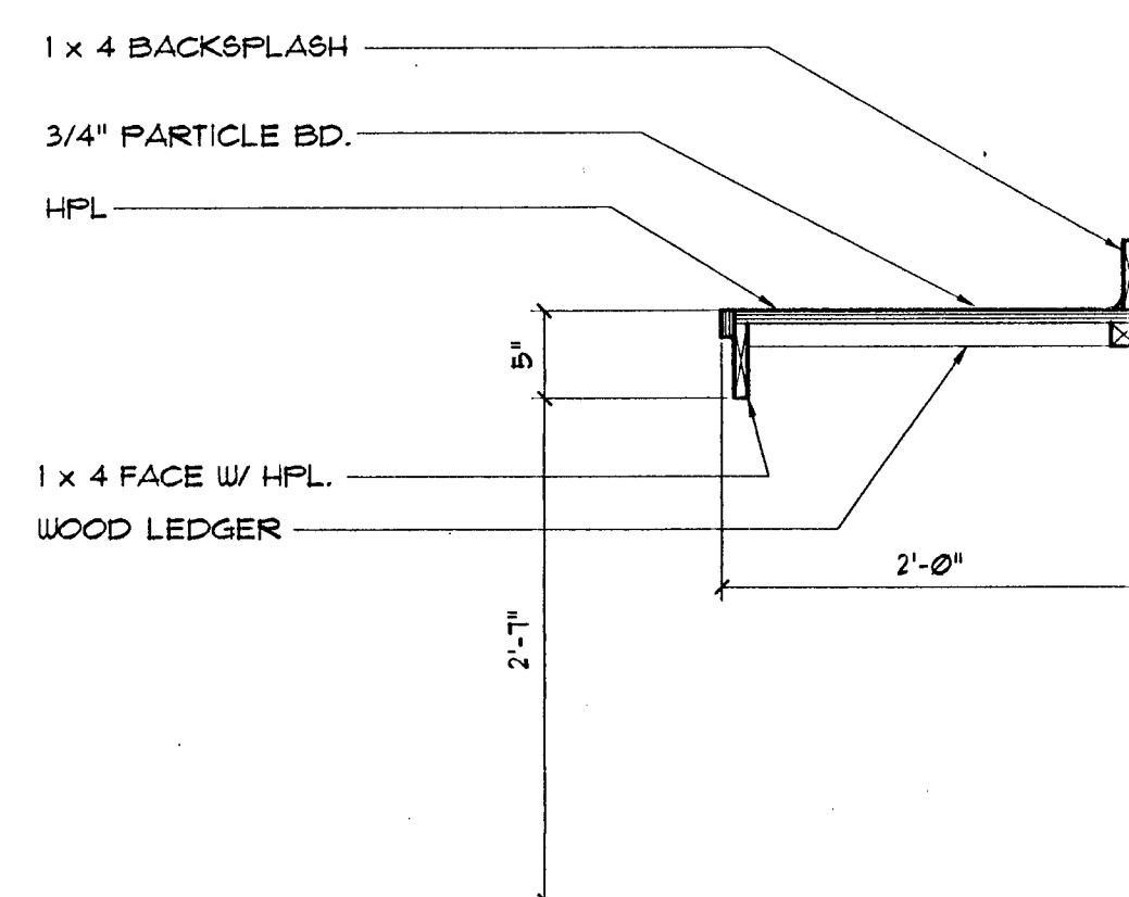
8 Phone Shelf Detail Scale: 1\"/>
