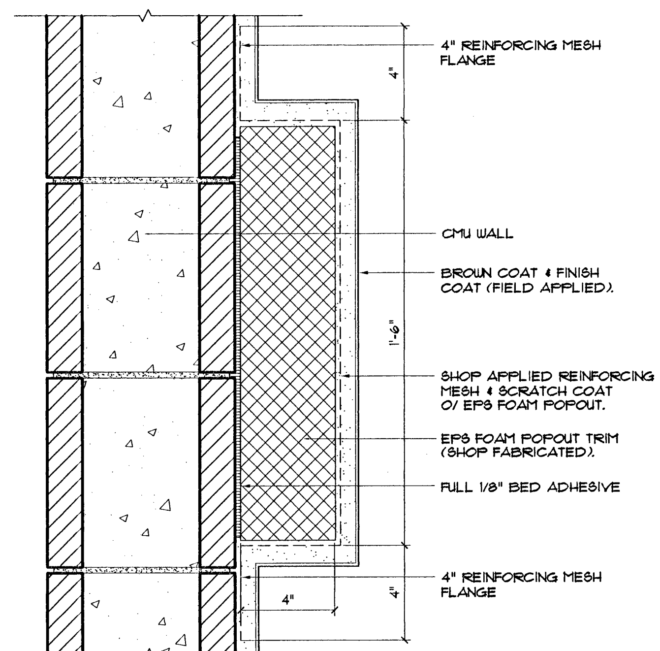
10 Foam Popout w/ Stucco Finish Scale: 3\"/>
