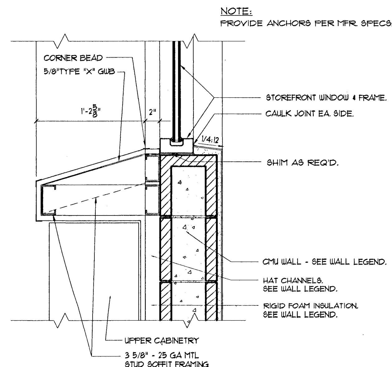
6 Sloped Window Sill Detail Scale: 1 1/2\"/>
