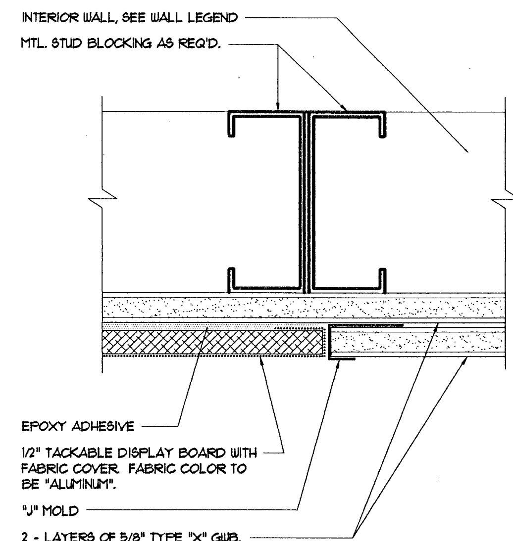
12 Display Board Detail Scale: 6\"/>
