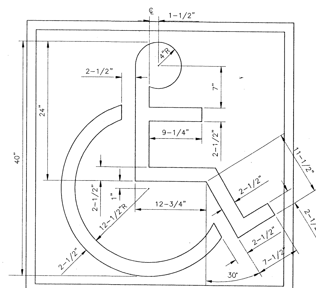
HANDICAP SYMBOL (C) N.T.S.
