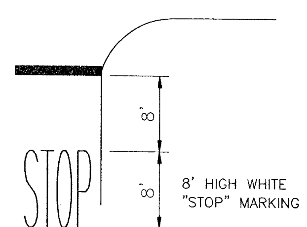
TYPICAL PAVEMENT MARKINGS (B) N.T.S.
