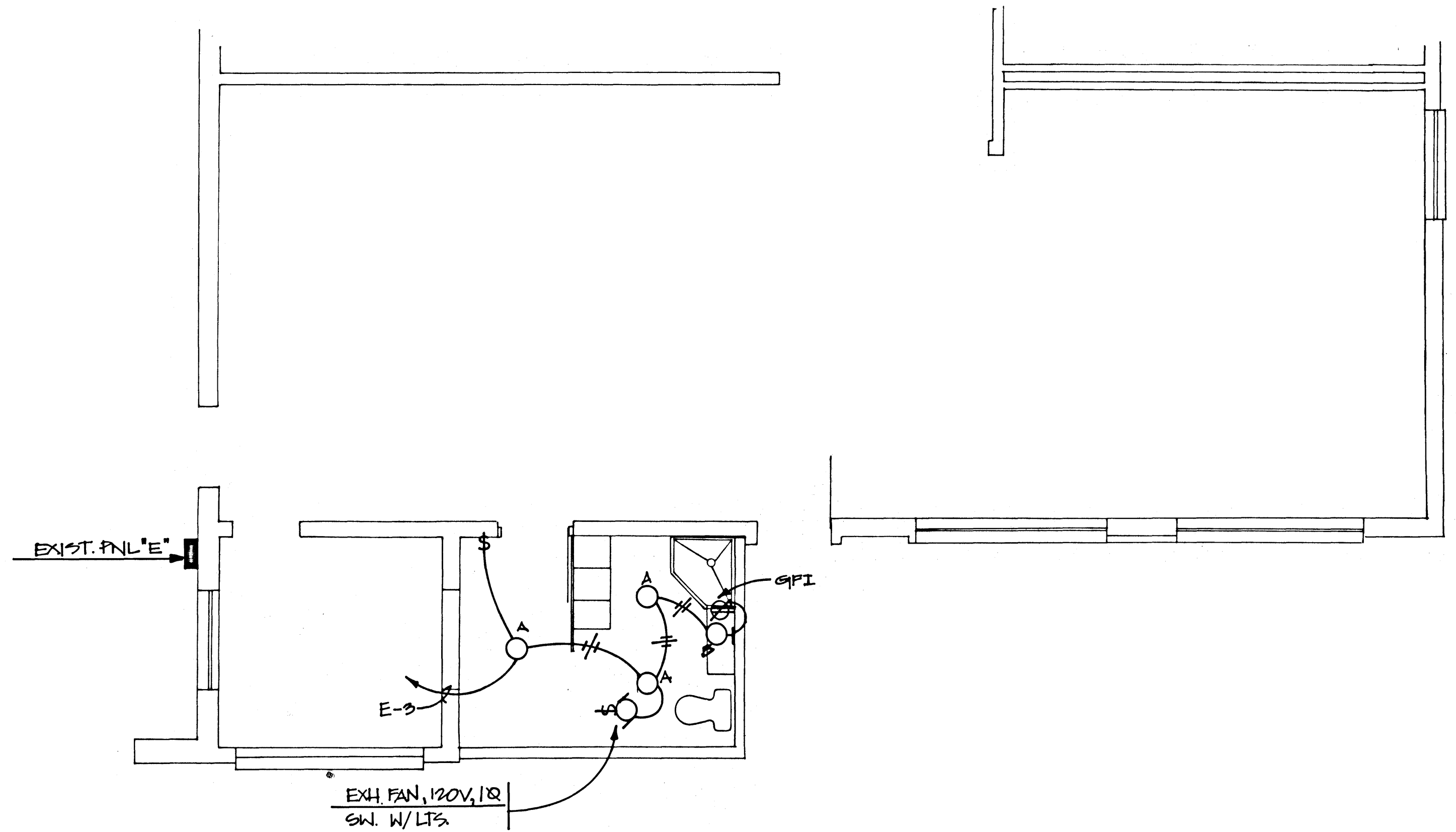
ELECTRICAL FLOOR PLAN SCALE: 1/4" 1'-0"
