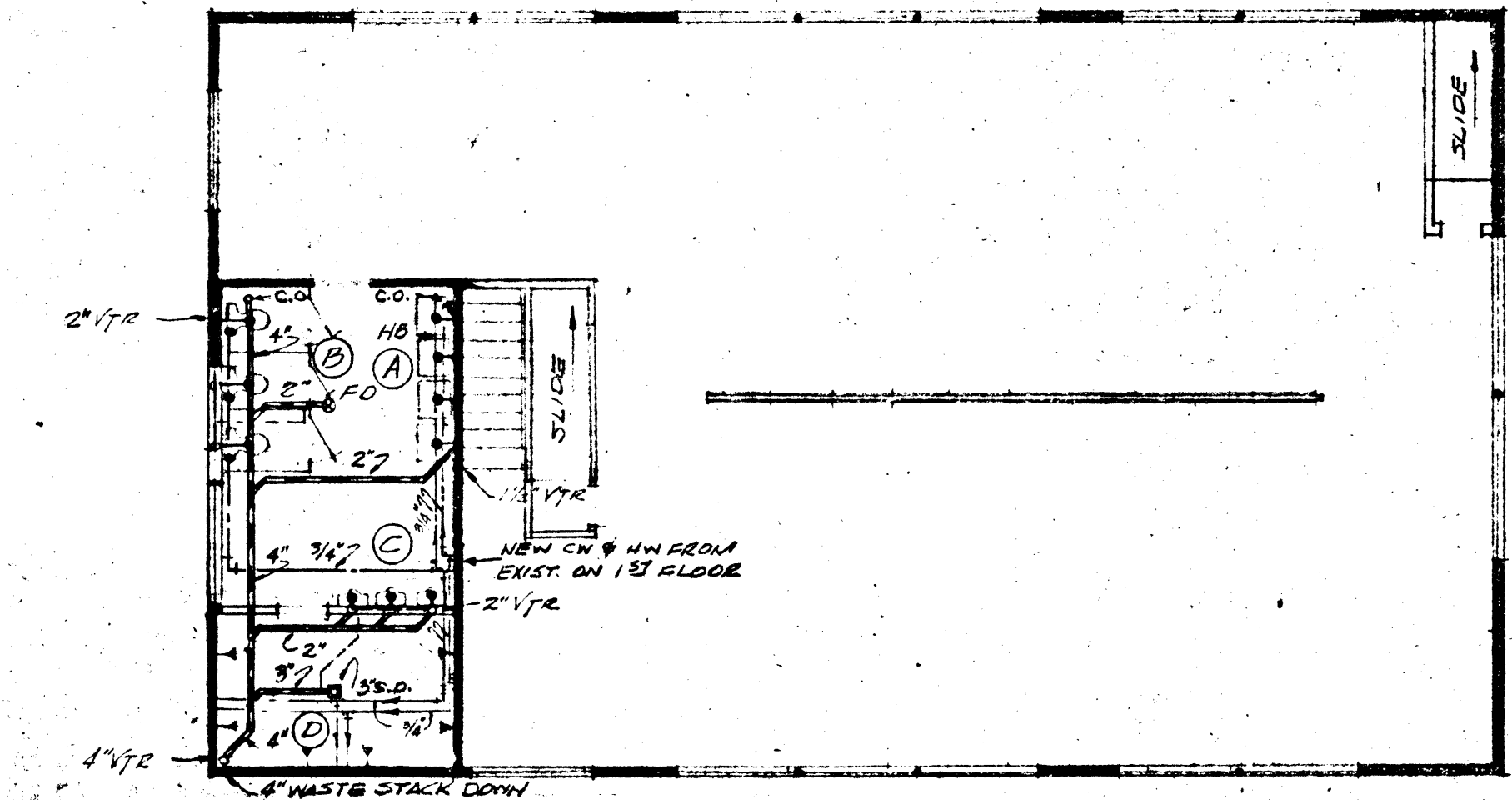
SOIL PIPING AT 2ND FLOOR NO SCALE
