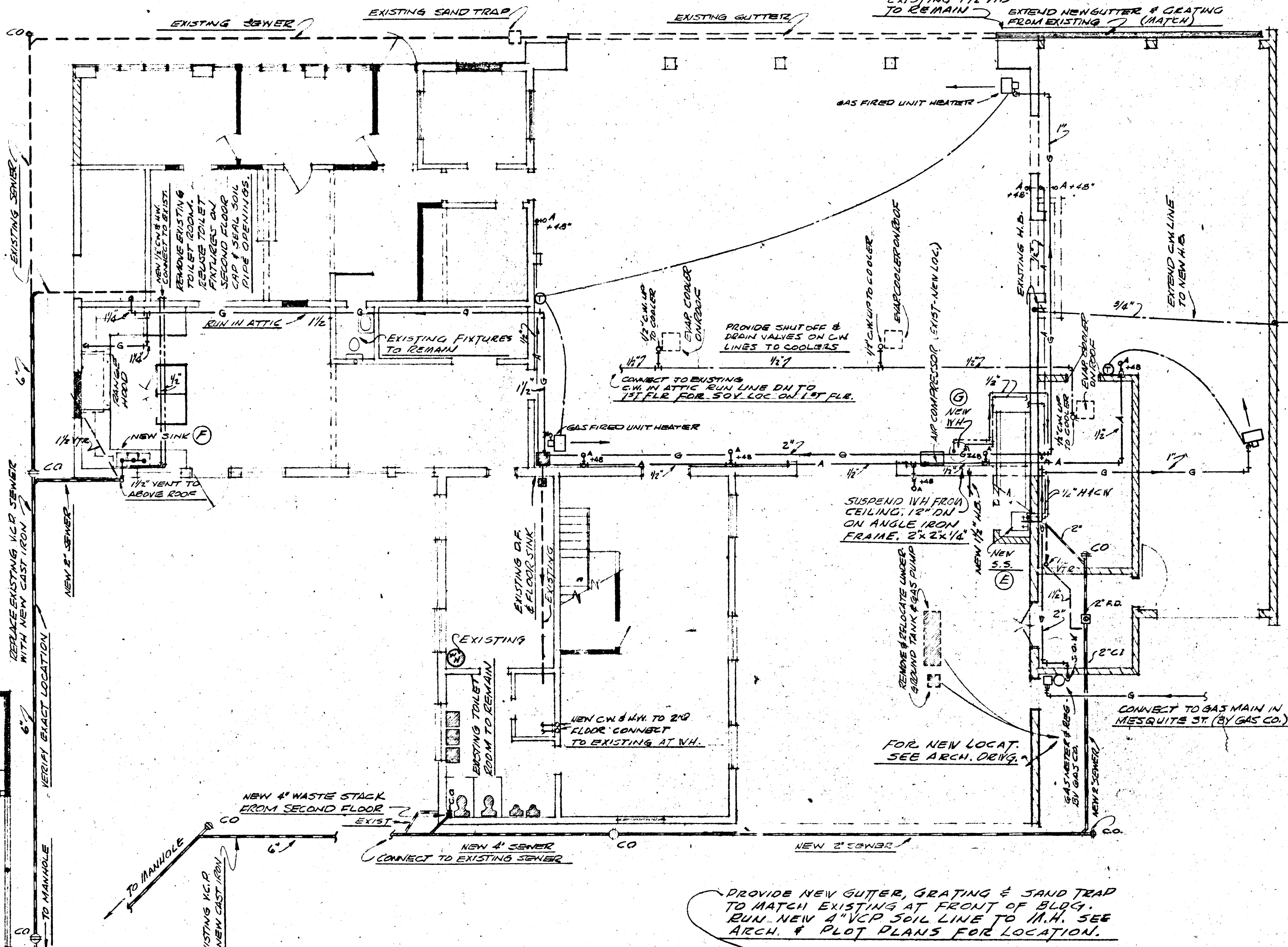
PLUMBING - FIRST FLOOR PLAN - 1/8" = 1'-0"
