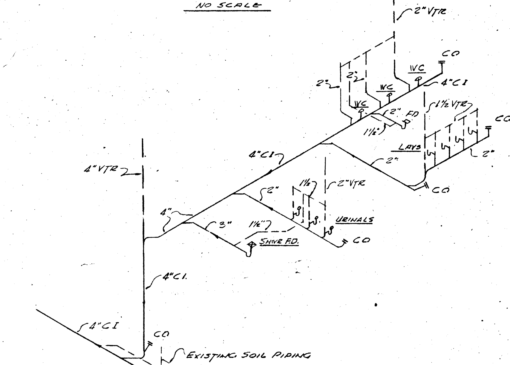
SOIL PIPING AT 2ND FLOOR NO SCALE
