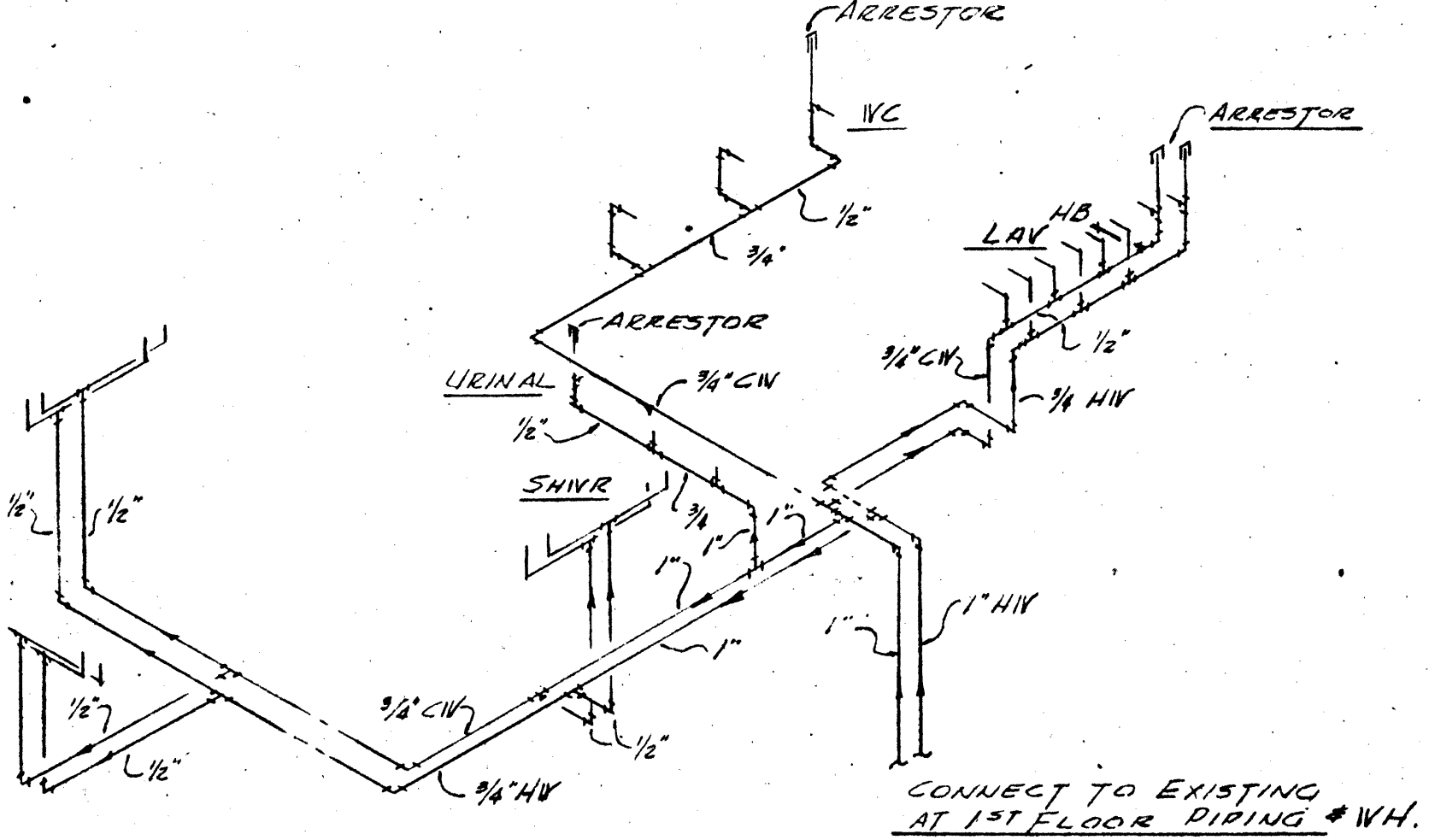
WATER PIPING AT 2ND FLOOR NO SCALE
