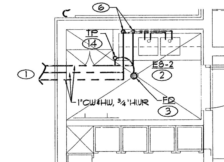
6 RESCUE CLEAN ROOM - DOMESTIC WATER SCALE: 1/4" = 1'-0"
