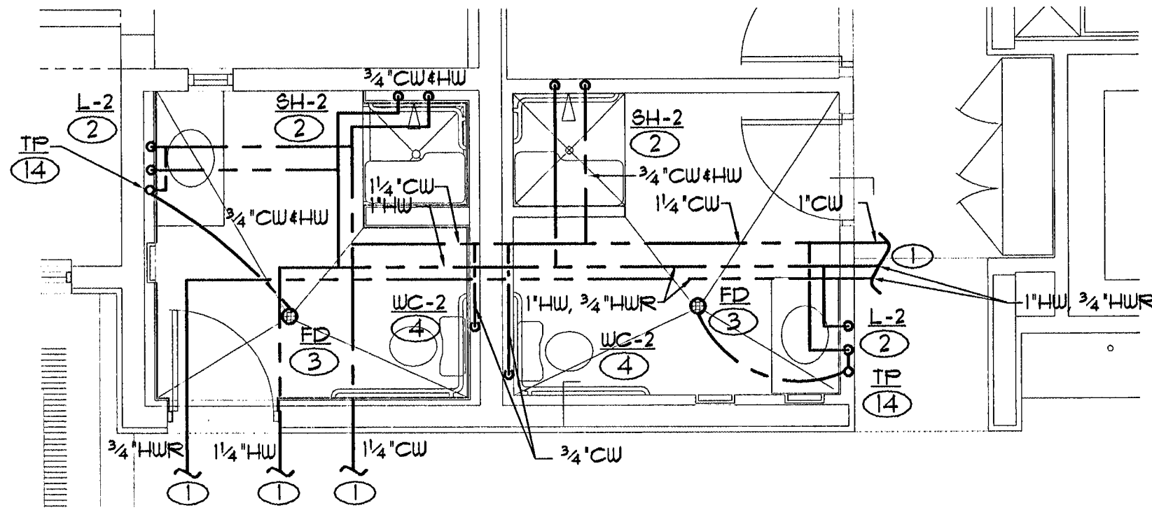
1 RESTROOM - DOMESTIC WATER SCALE: 1/4" = 1'-0"
