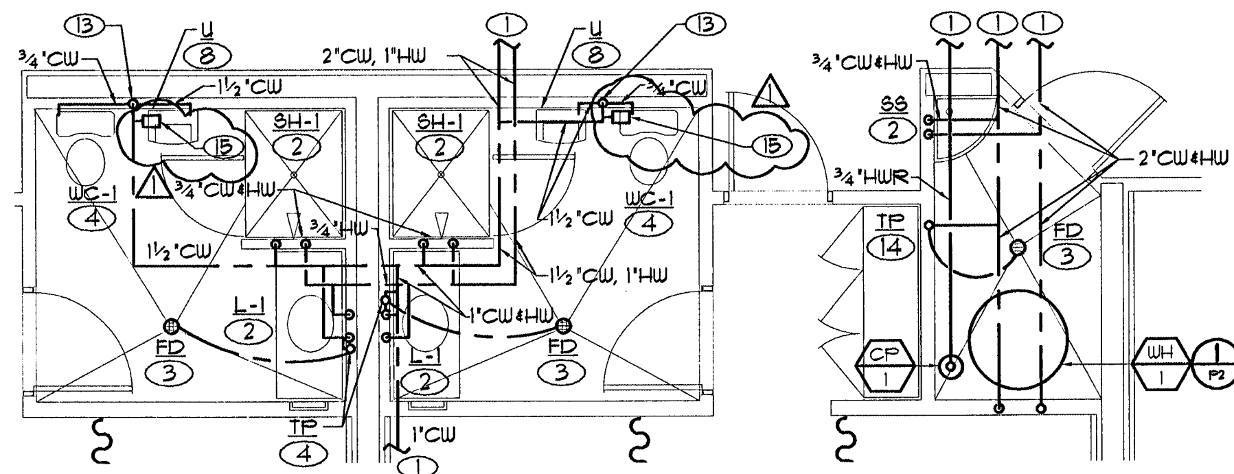
4 RESTROOM - DOMESTIC WATER SCALE: 1/4" = 1'-0"
