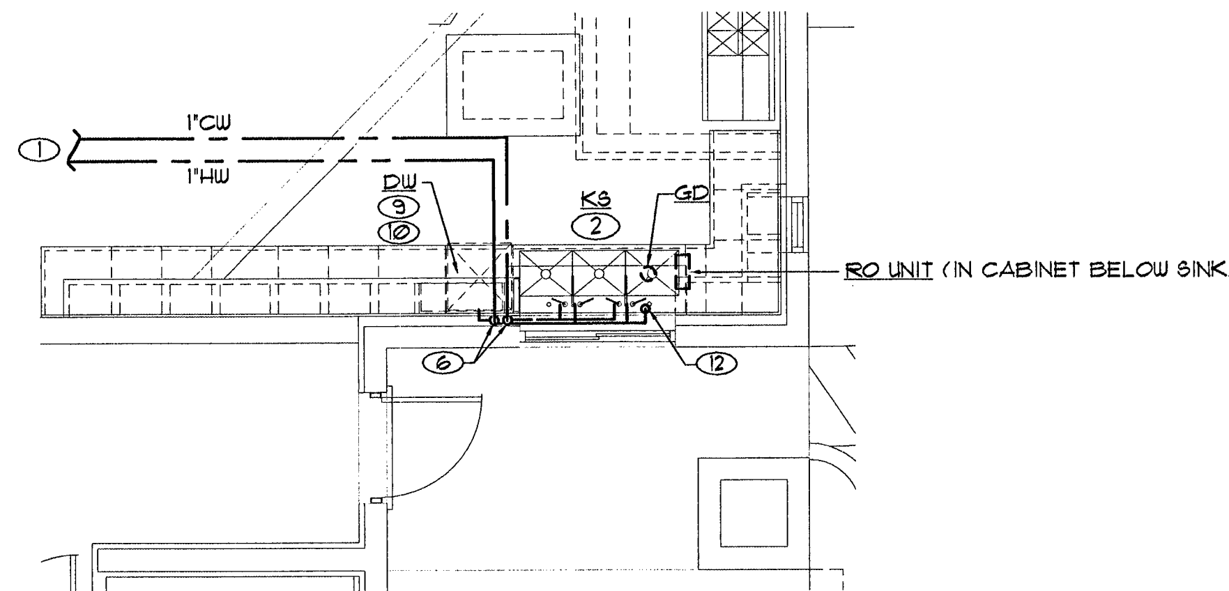
5 KITCHEN - DOMESTIC WATER SCALE: 1/4" = 1'-0"
