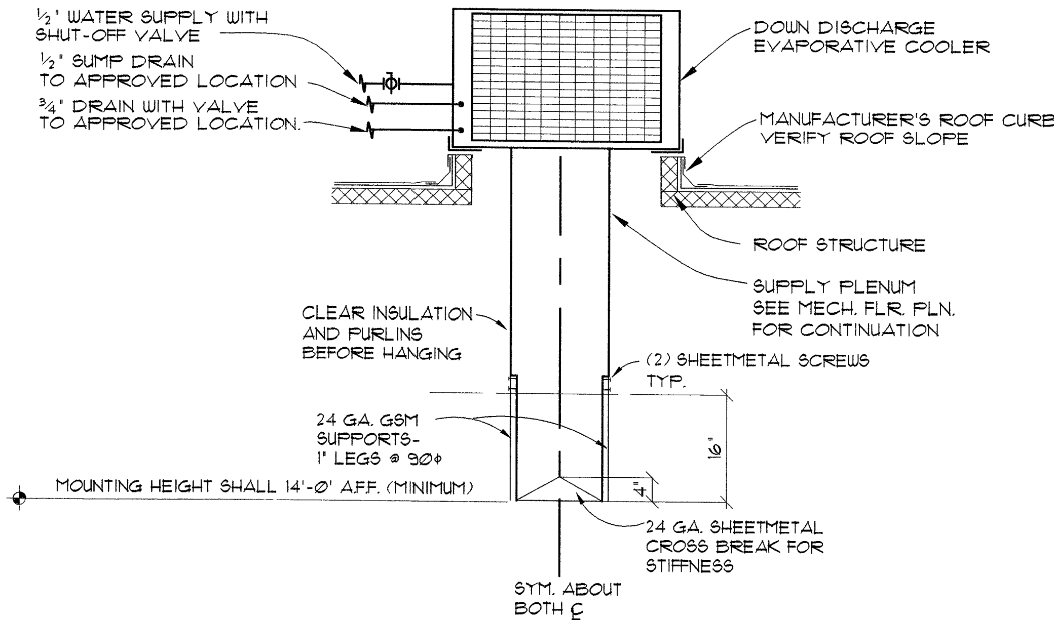
EVAPORATIVE COOLER UNIT DETAIL NO SCALE
