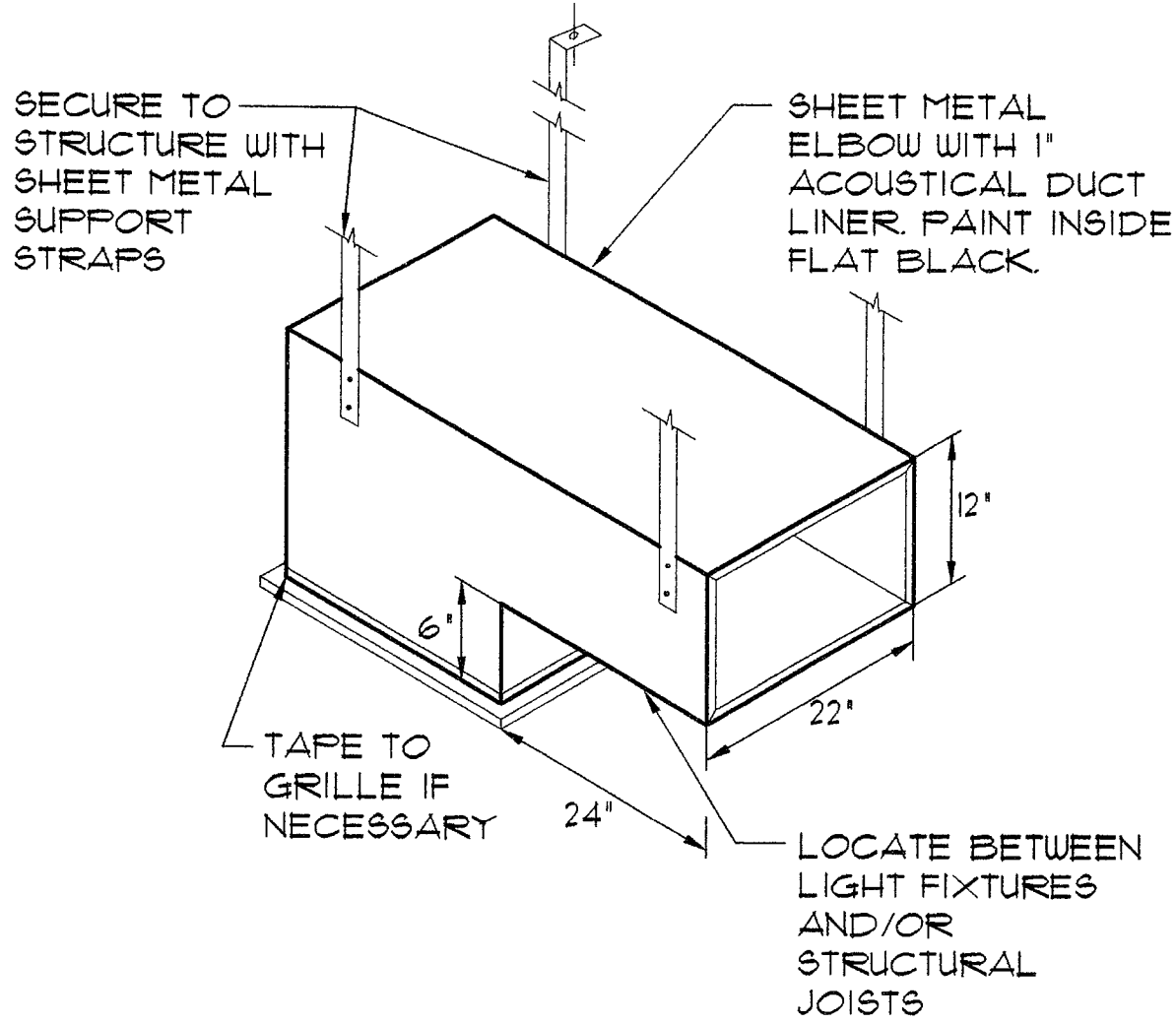
RETURN AIR GRILLE DETAIL NO SCALE
