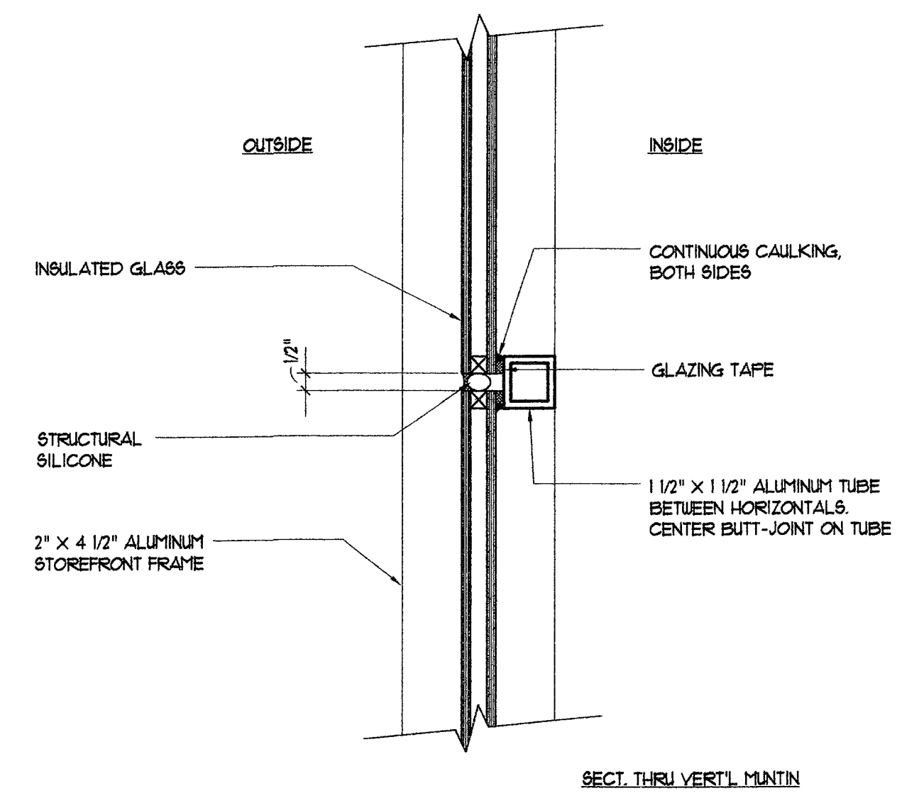
10 Butt Glazing Detail Scale: 3/4"=1'-0" AT-010
