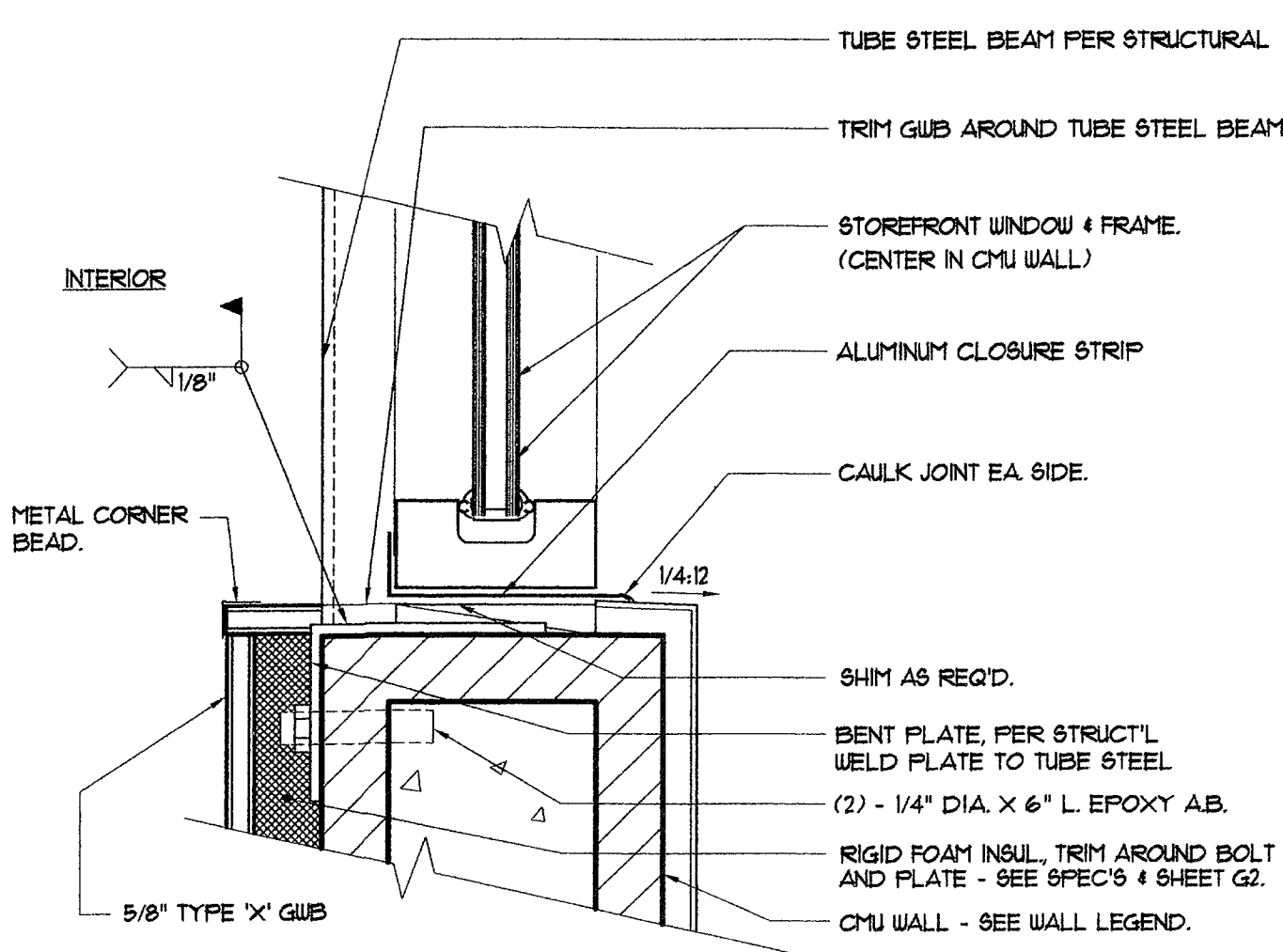
6 T.S. Support @ Sill of Window "I" Scale: 3/4"=1'-0" AT-006
