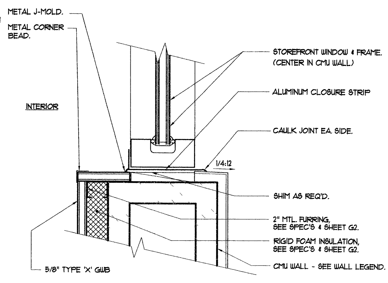
7 Exterior Window Sill Detail Scale: 3/4"=1'-0" AT-007
