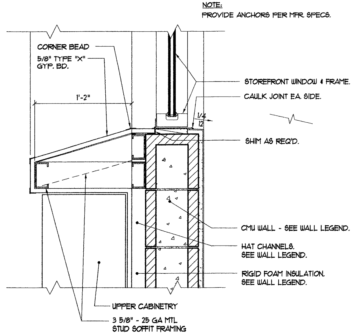
1 Sloped Window Sill Detail Scale: 1/2"=1'-0" AT-001
