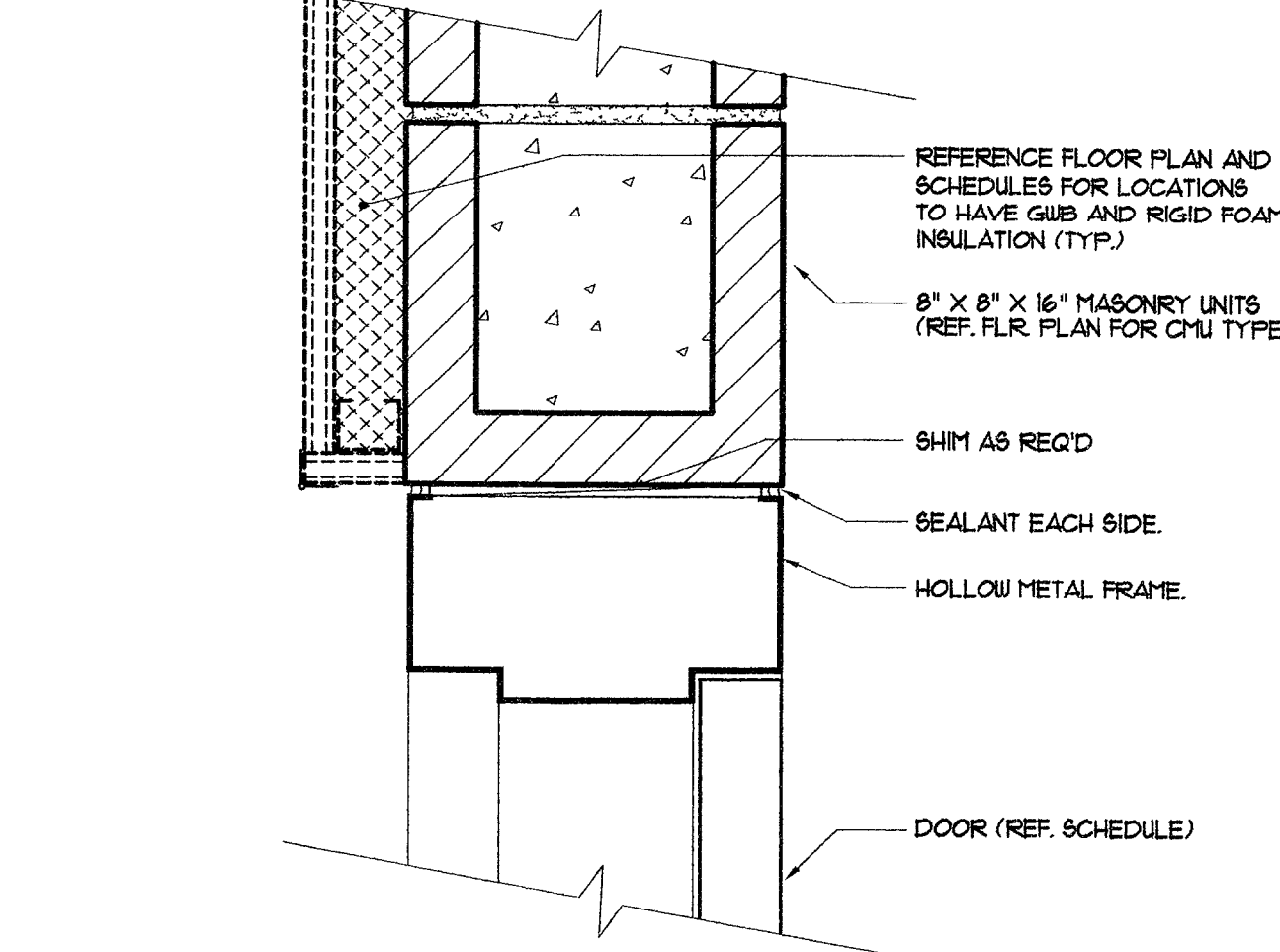
3 Interior Door Head / Jamb (Sim.) Scale: 3/4"=1'-0" 08100-16 AT-003
