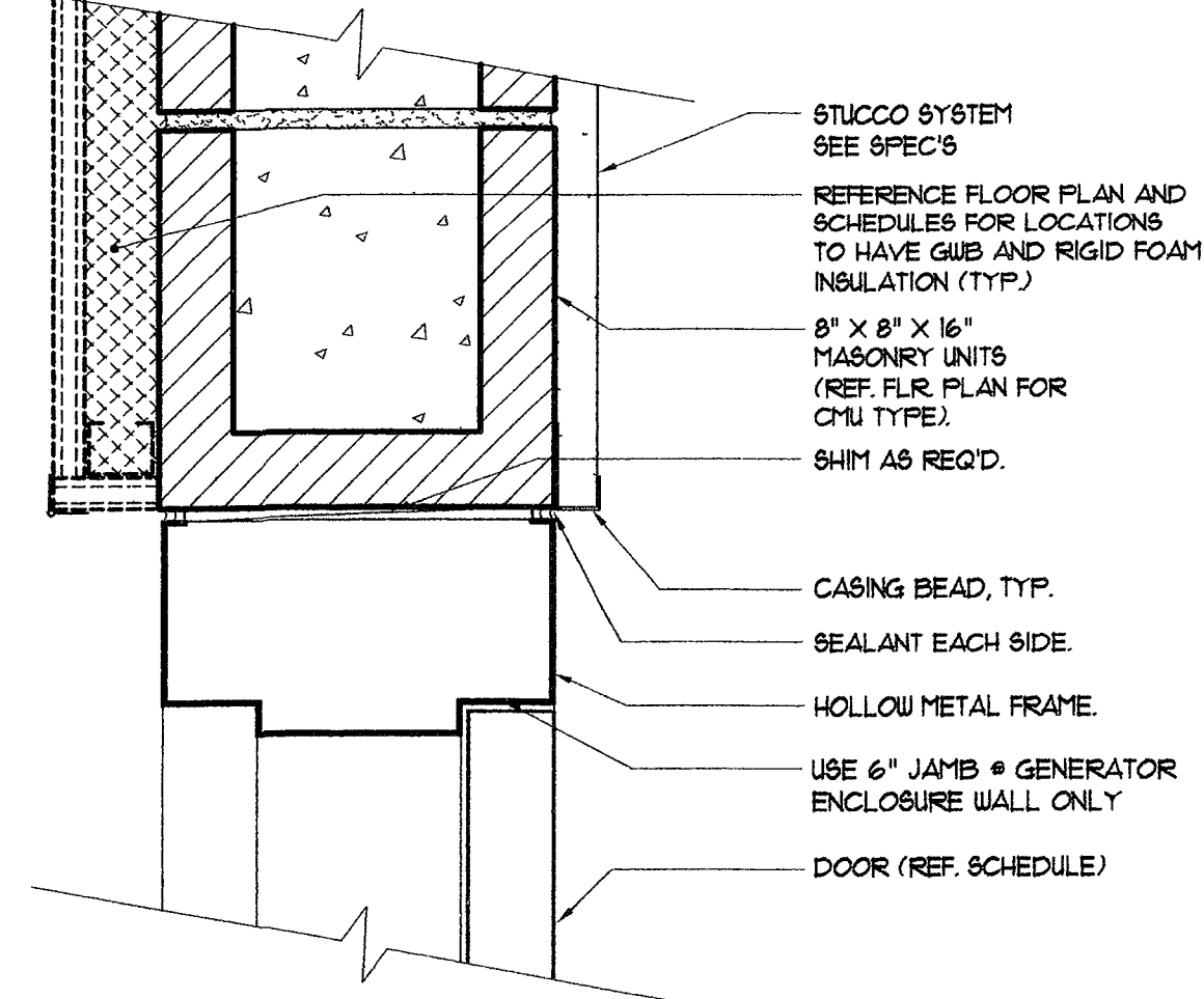
2 Head - Jamb @ Exterior Door Scale: 3/4"=1'-0" 08100-15 AT-007
