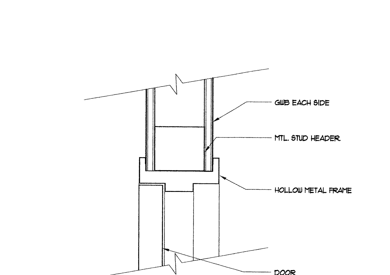
4 Interior Door Head - Jamb Sim. Scale: 3/4"=1'-0" 08100-03 AT-004
