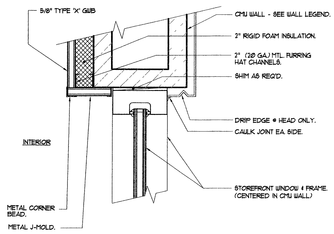
5 Exterior Window Jamb/ Head Detail Scale: 3/4"=1'-0" 08500-34 AT-005
