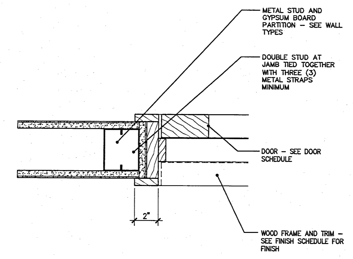
JAMB 2 SCALE : 3" = 1'-0" 723d02.dwg
