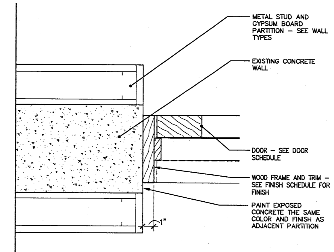
JAMB 4 SCALE : 3" = 1'-0" 723d03.dwg
