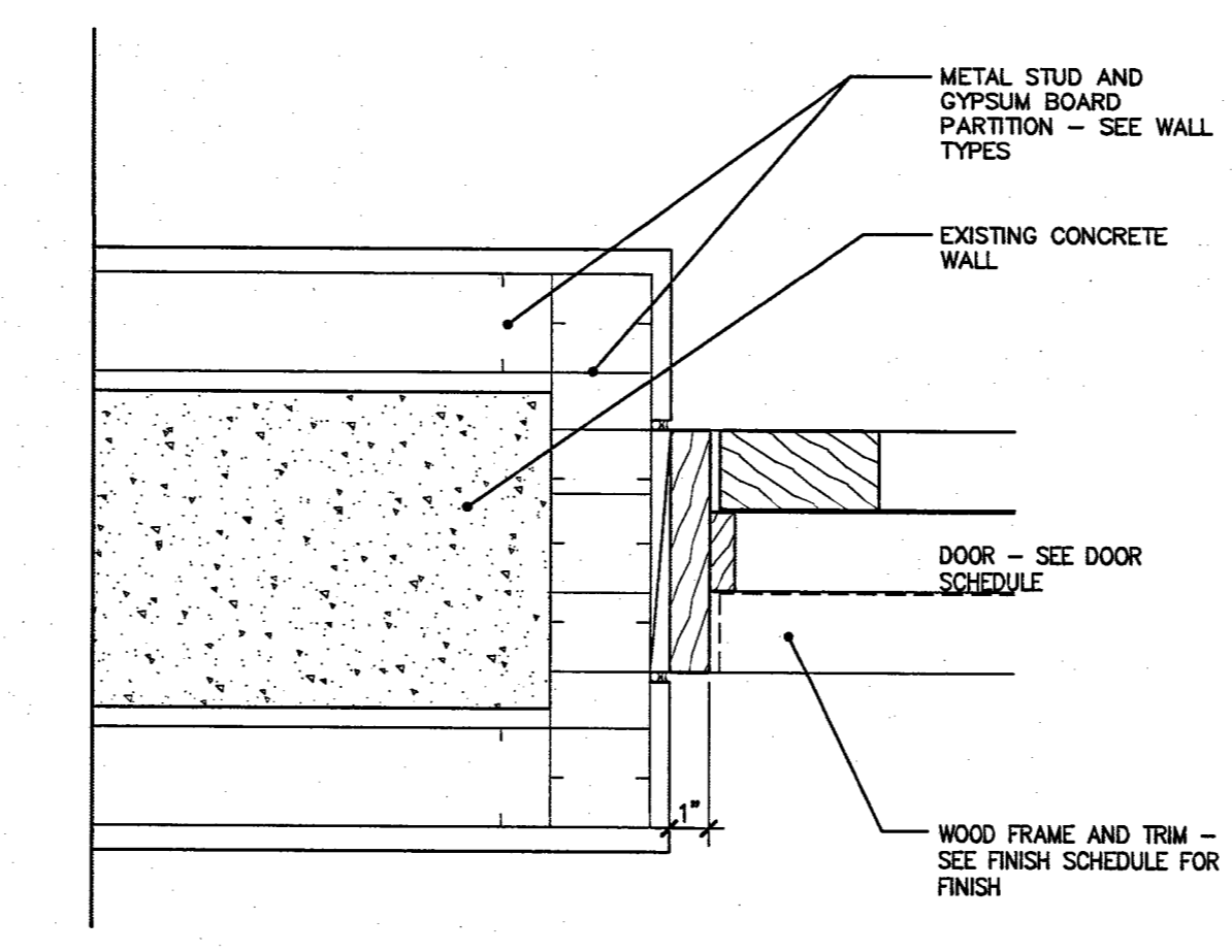
JAMB 5 SCALE : 3" = 1'-0" 723d05.dwg
