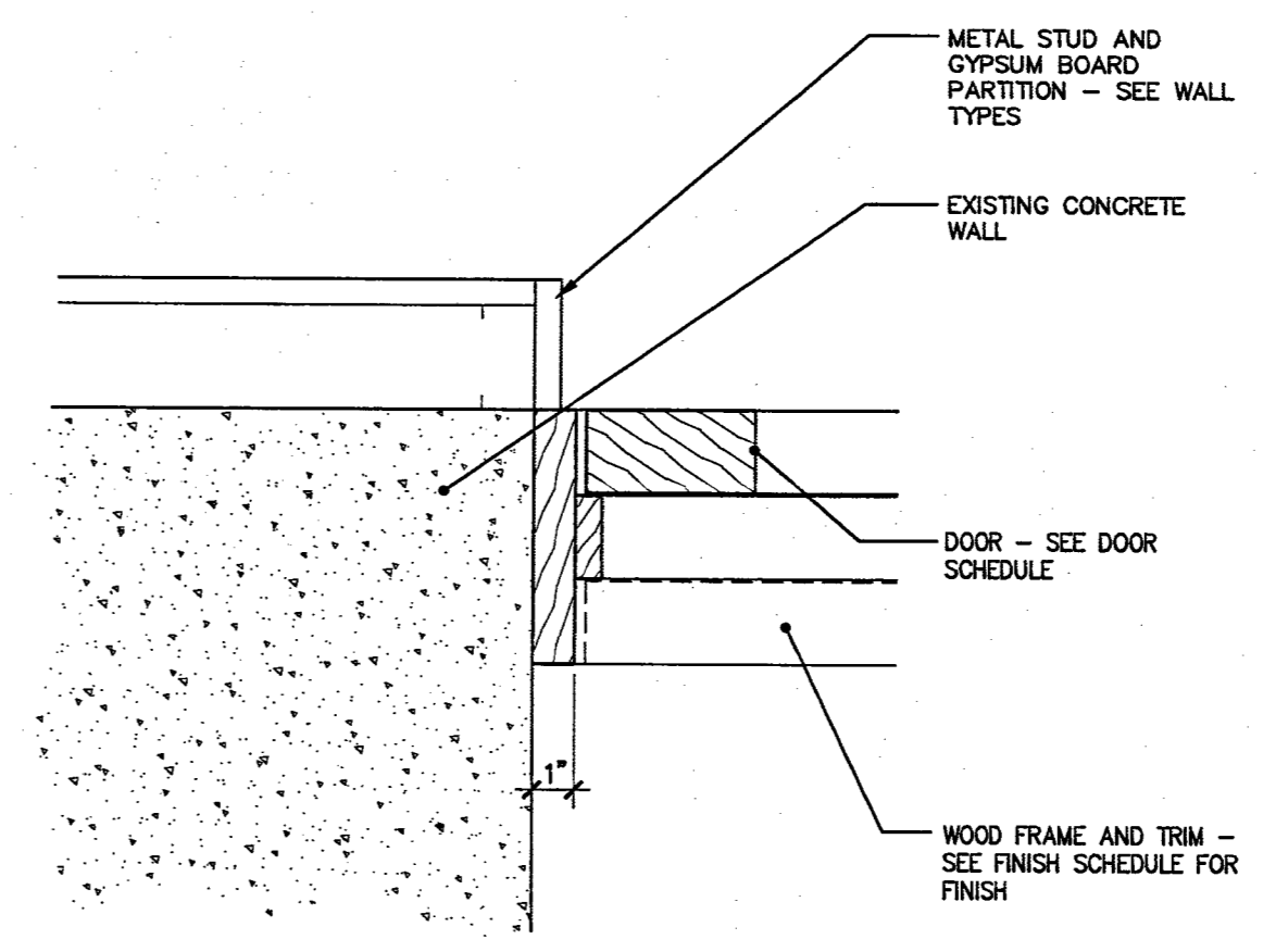
JAMB 3 SCALE : 3" = 1'-0" 723d03.dwg
