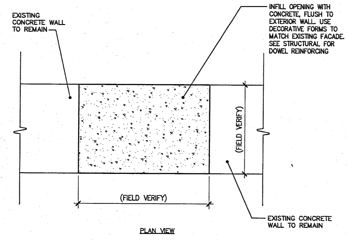
INFILL CONCRETE 7 SCALE : 3" = 1'-0" 723d07.dwg
