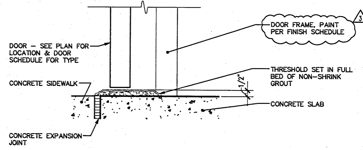
SILL DETAIL 6 SCALE : 3" = 1'-0" 723d06.dwg
