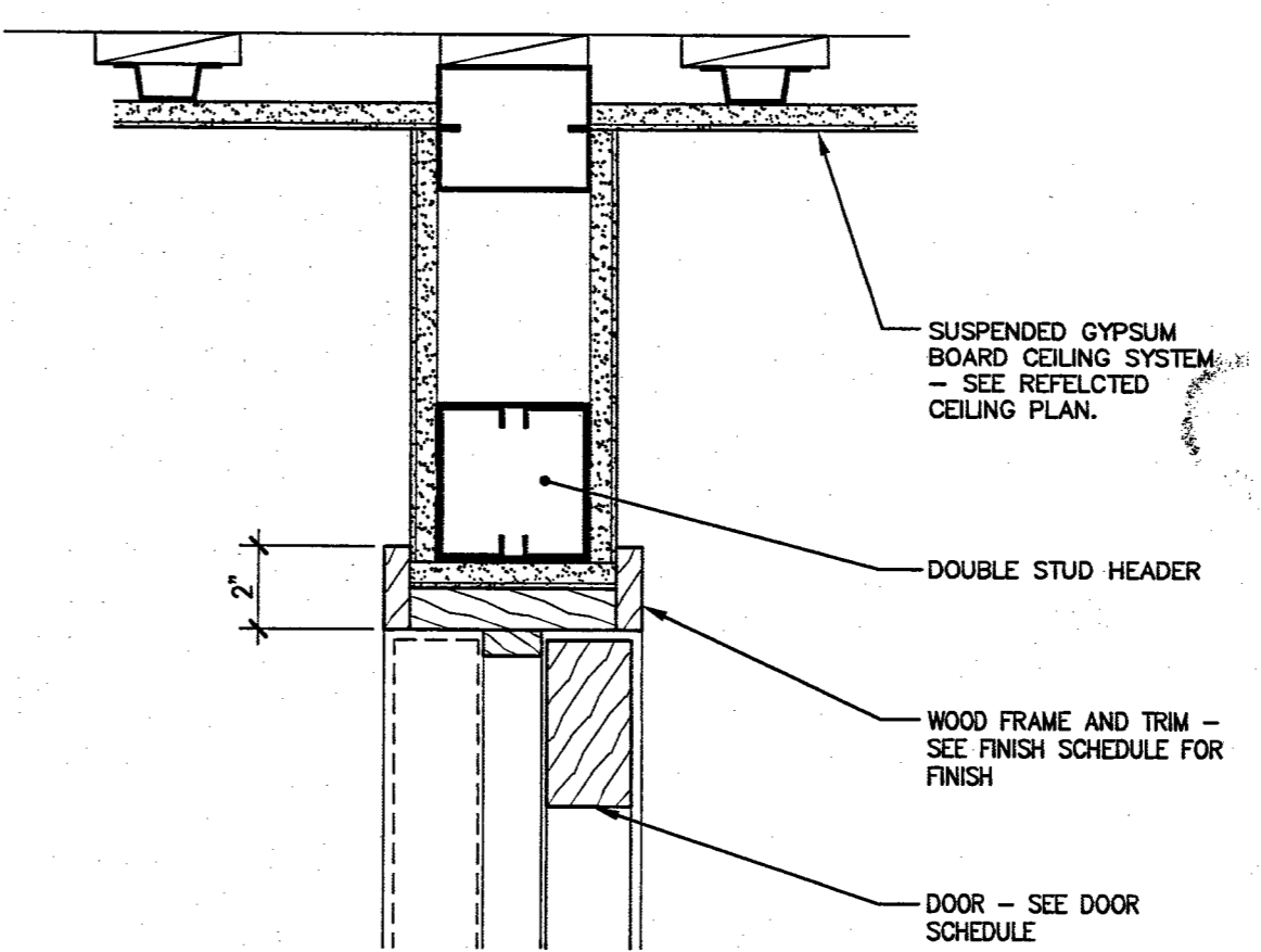
HEAD 1 SCALE : 3" = 1'-0" 723d01.dwg
