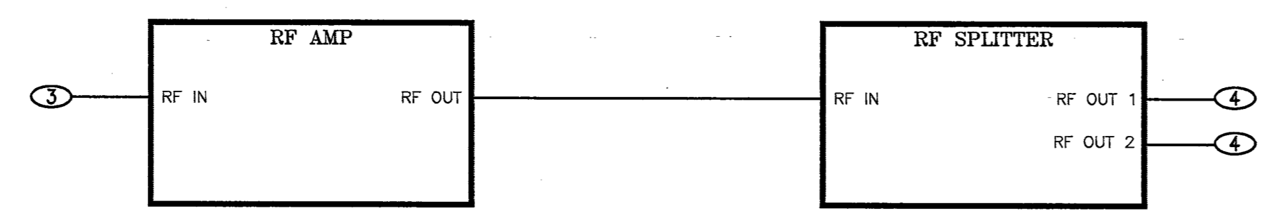
AUDITORIUM & CONFERENCE ROOM CATV C SCALE: NO SCALE TA0.03
