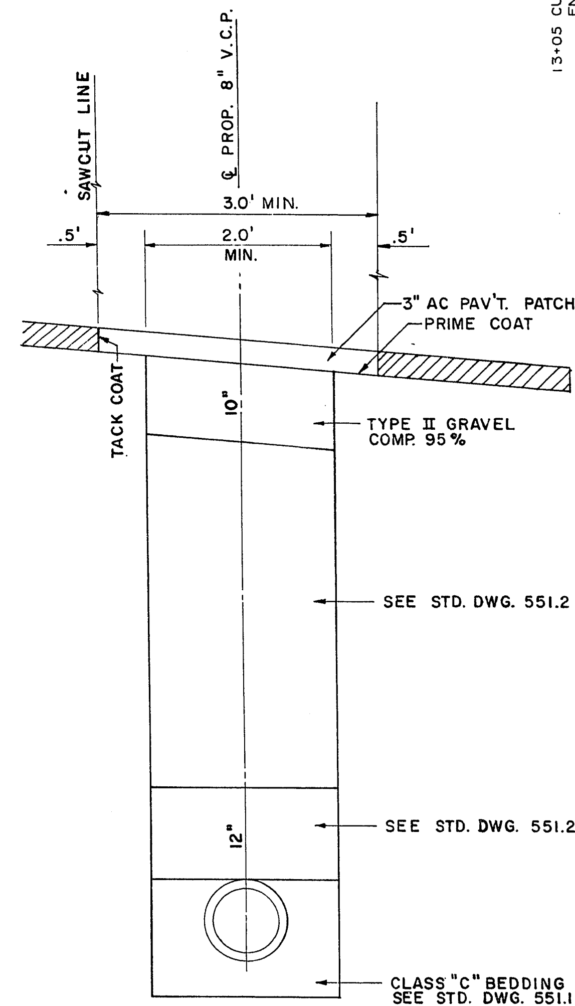
TYPICAL SECTION SCALE - 1"=1'
