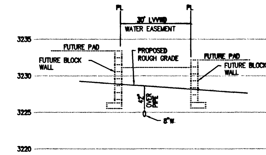
LVWD EASEMENT SECTION N.T.S.
