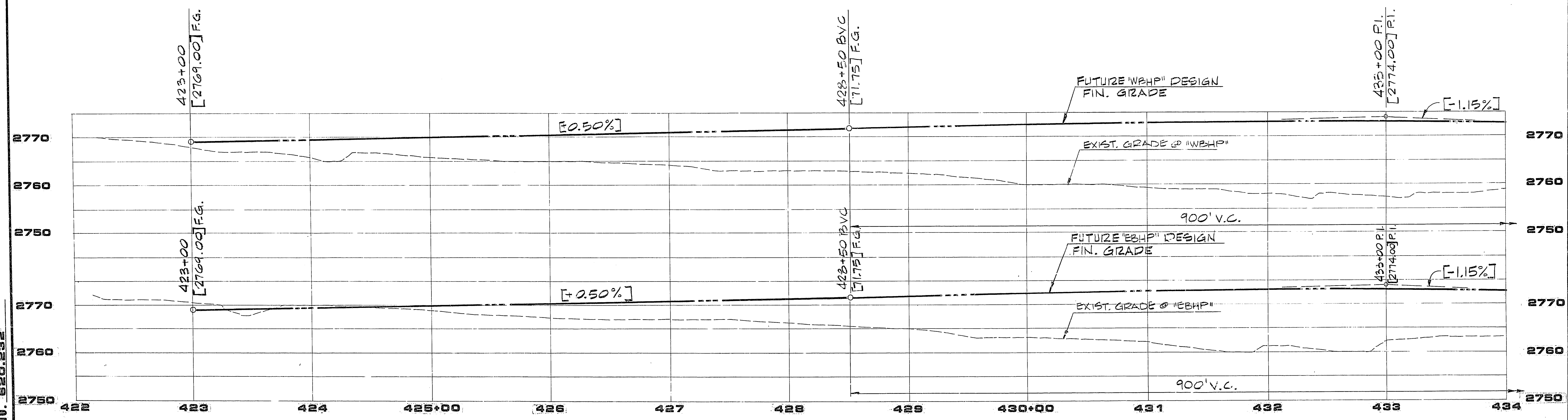
PROFILE SCALE: HORIZ: 1" = 40' VERT: 1" = 10'
