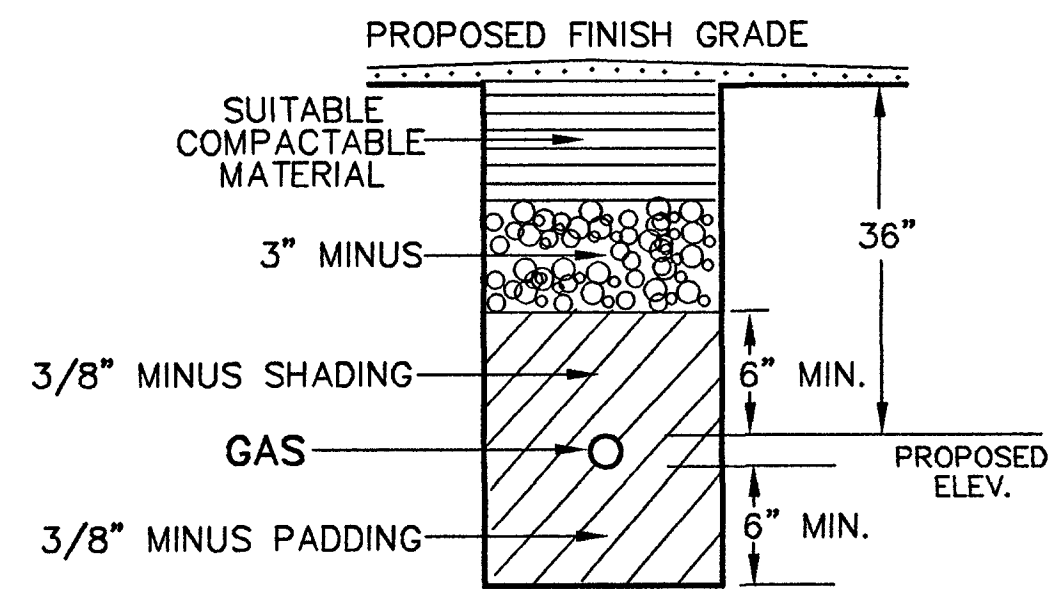
TRENCH DETAIL IMPROVED AREAS ONLY NOT TO SCALE CITY OF LAS VEGAS
