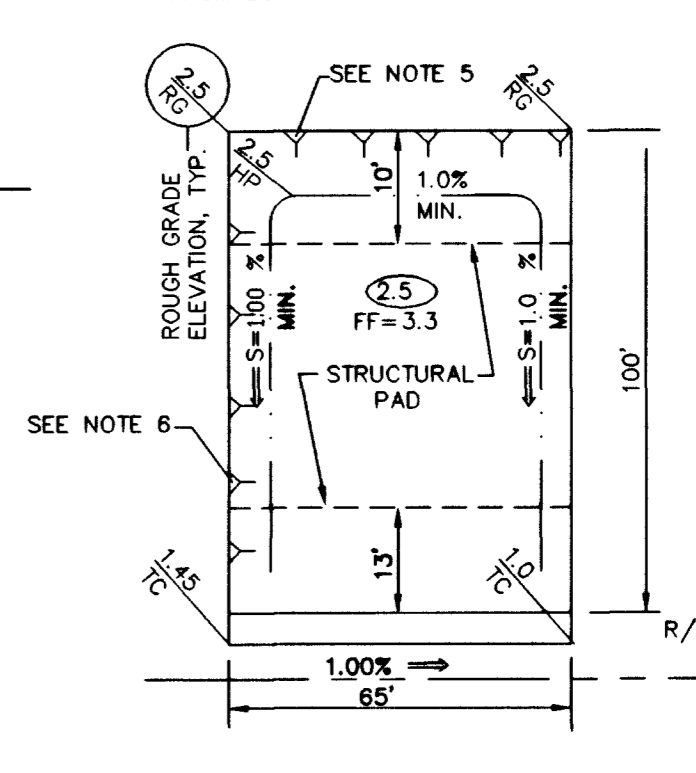
TYPICAL GRADING PLAN
