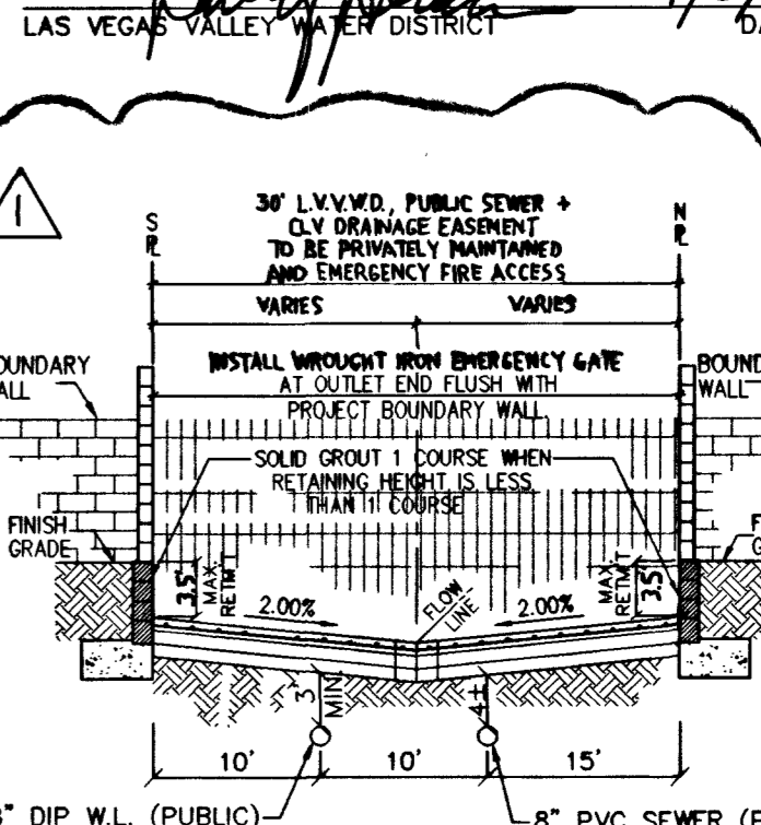
36' PUBLIC DRAINAGE EASEMENT DETAIL & L.V.V.W.D. UTILITY CLEARANCE DETAIL (N.T.S.)
