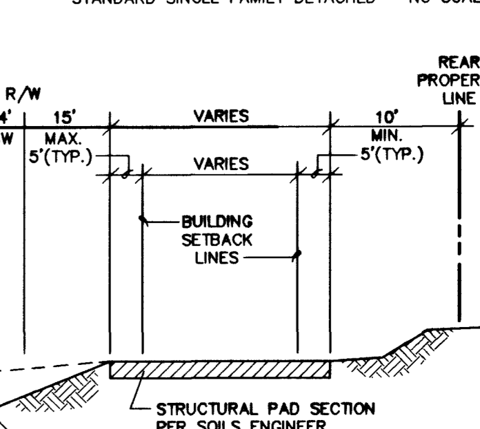
TYPICAL GRADING SECTION
