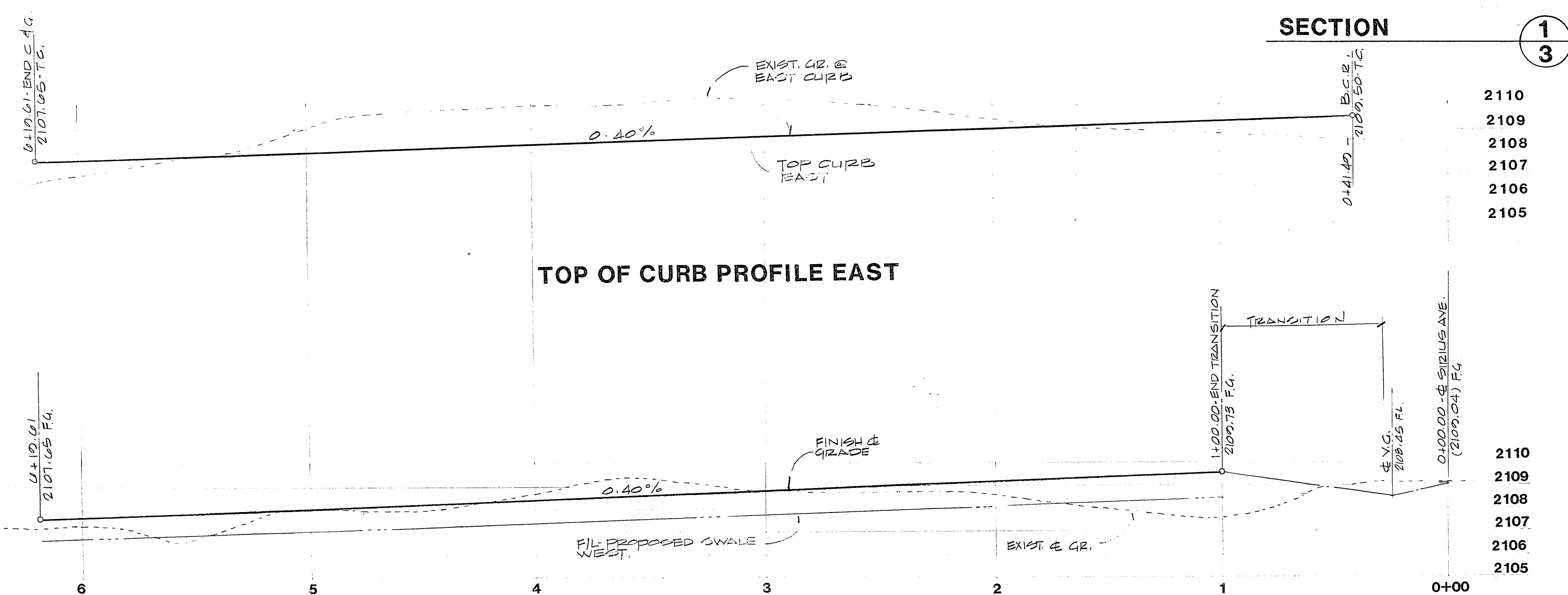
PROFILE - RIGEL AVENUE (SEE PLAN SHEET 2)
