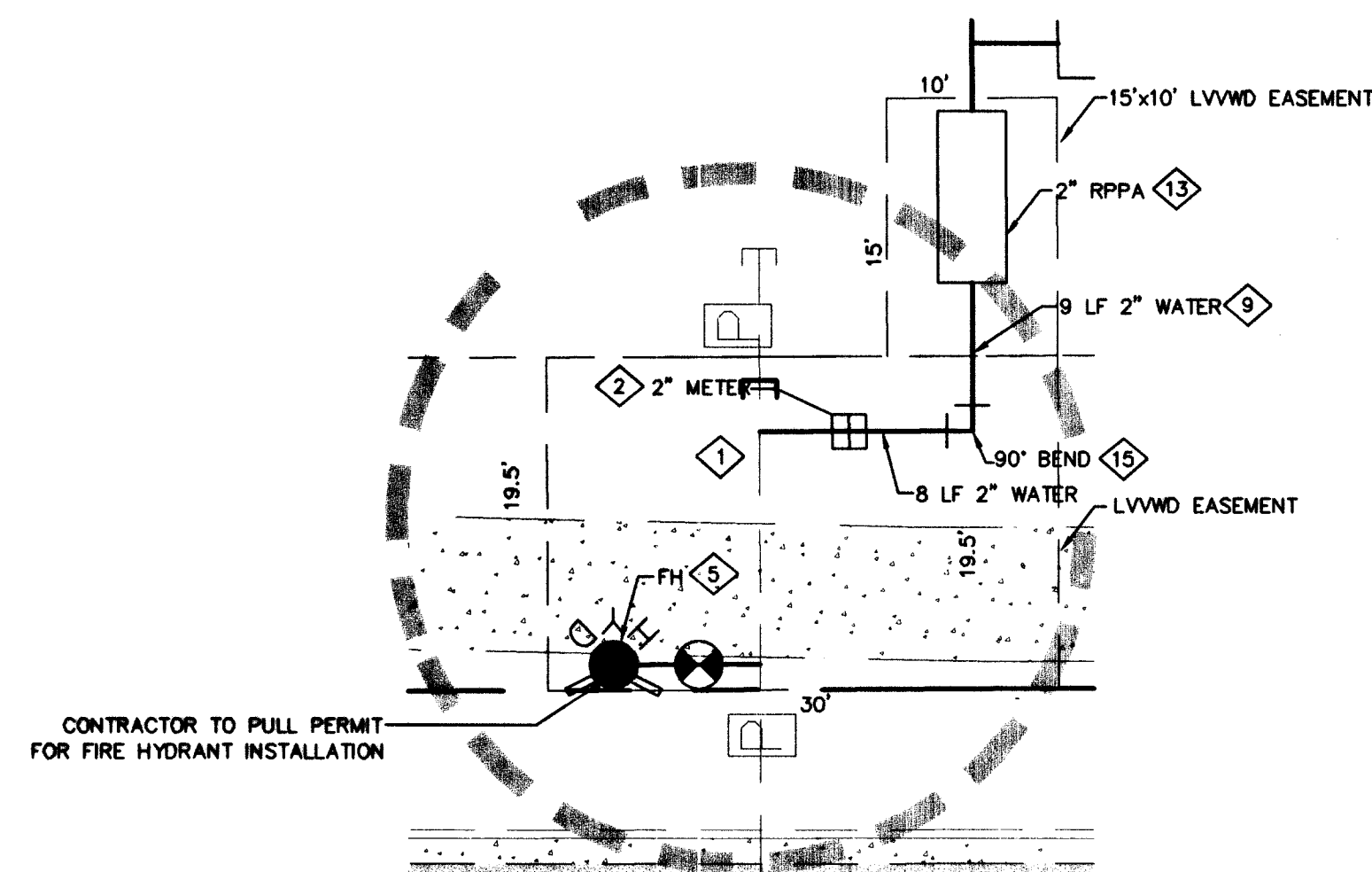
UTILITY EASMENT DETAIL "B"
