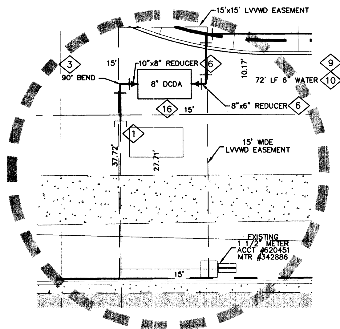
UTILITY EASMENT DETAIL "A"
