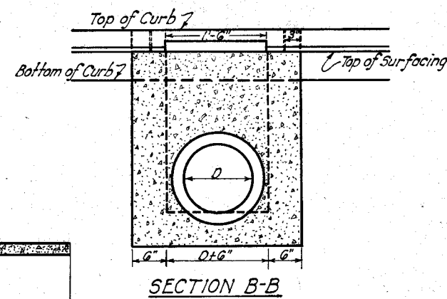
TYPICAL CURB INLET
