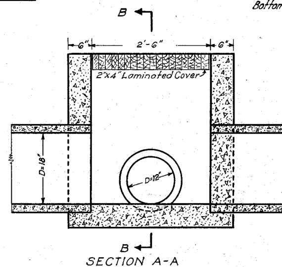
CLEANOUT BOX
