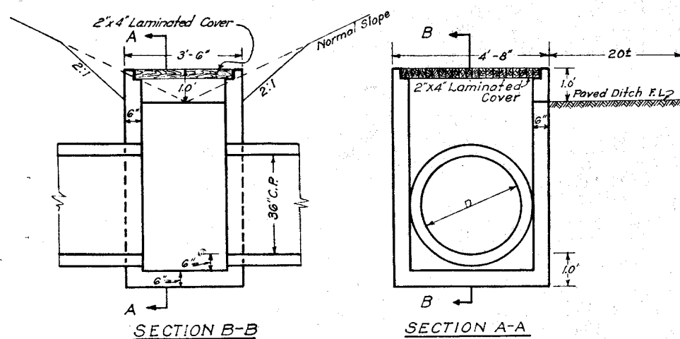
SPECIAL DROP BOX
