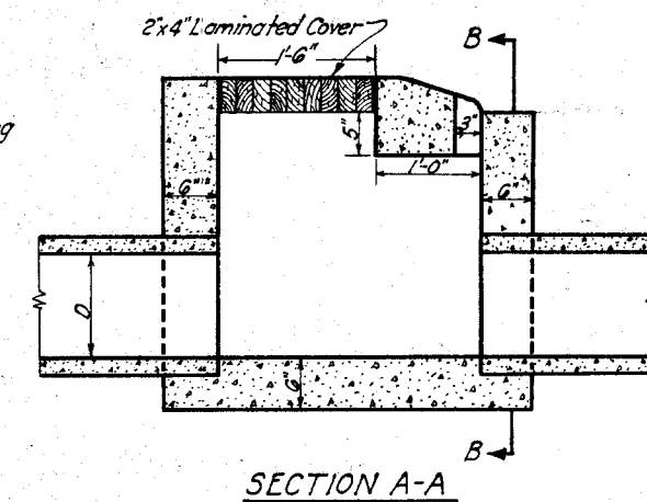
TYPICAL CURB INLET
