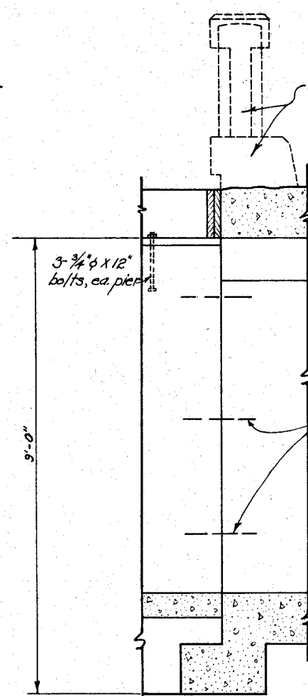
SECTION C-C
