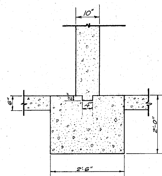
PIER FOOTINGS
