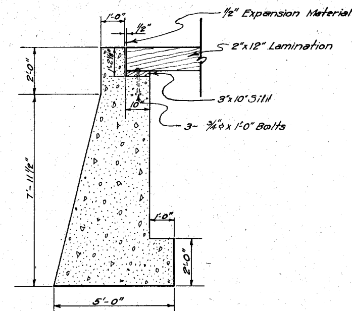
ABUTMENT WALL
