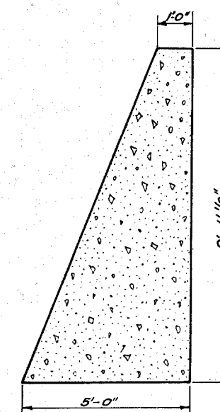
WING WALL
