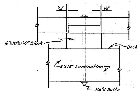
WHEEL GUARD SPLICE
