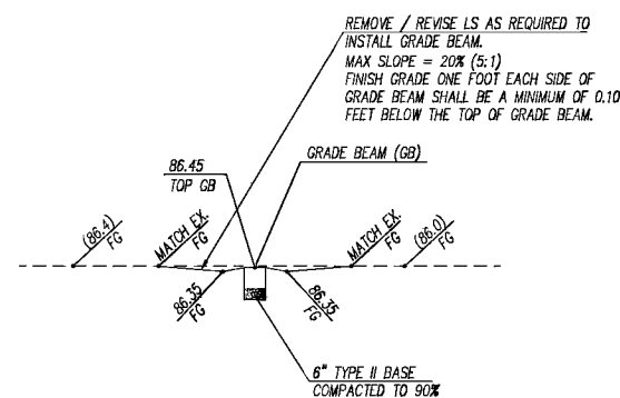
NTS TYPICAL CROSS-SECTION THROUGH GRADE BEAM IN EXISTING LANDSCAPE AREA A C8.00
