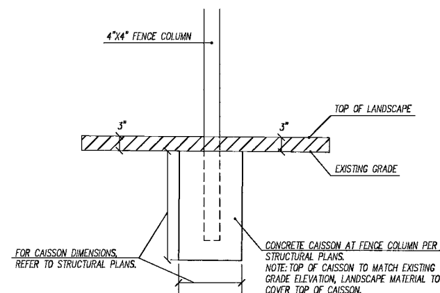
NTS TYPICAL CROSS-SECTION OF FENCE COLUMN CAISSON IN PAVEMENT AREA C C8.00
