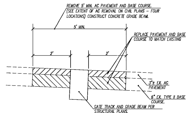
NTS TYPICAL CROSS-SECTION OF ASPHALT REMOVAL AND REPLACEMENT AT GATE TRACK AND GRADE BEAM LOCATIONS B C8.00
