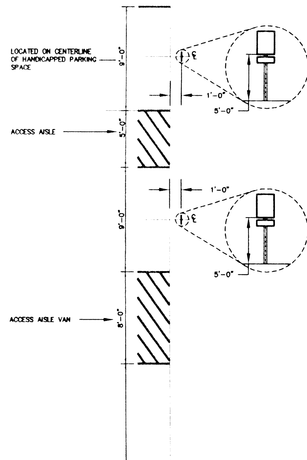
DETAIL B
