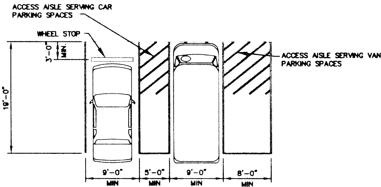
DETAIL A
