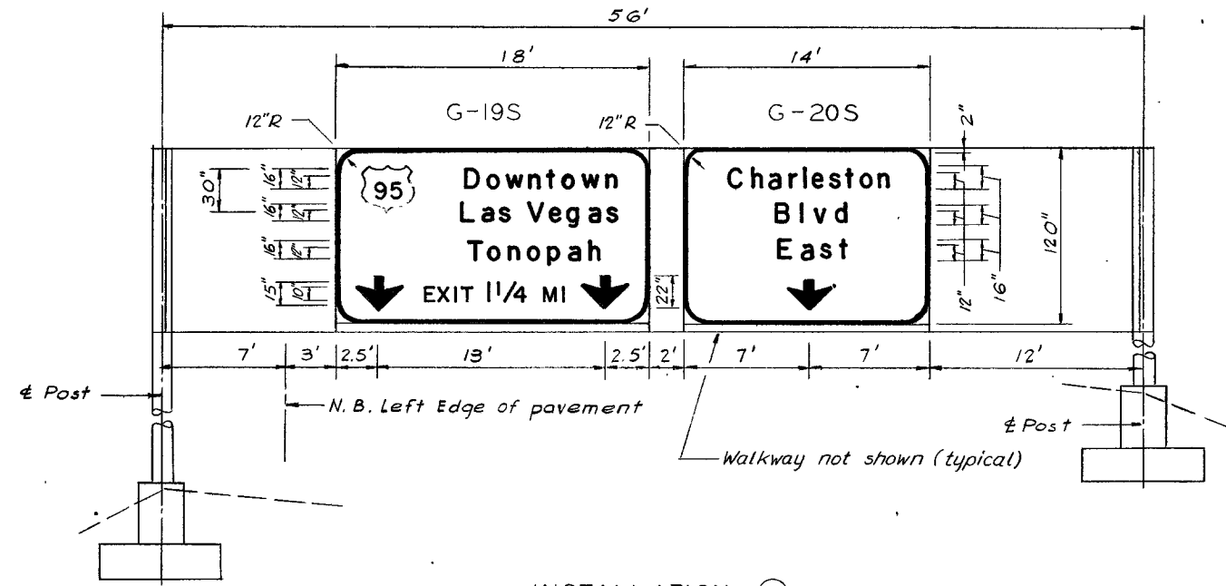
INSTALLATION ㉓
