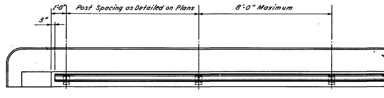
PART PLAN
