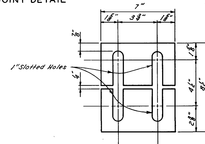
SHIM DETAIL
