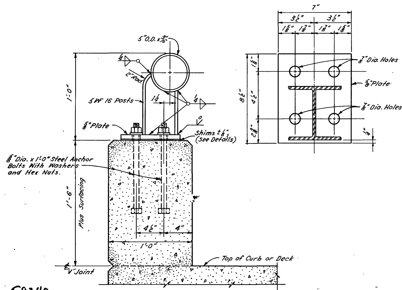
RAILING DETAILS
