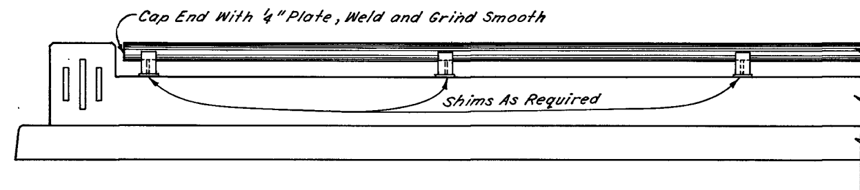
PART ELEVATION
